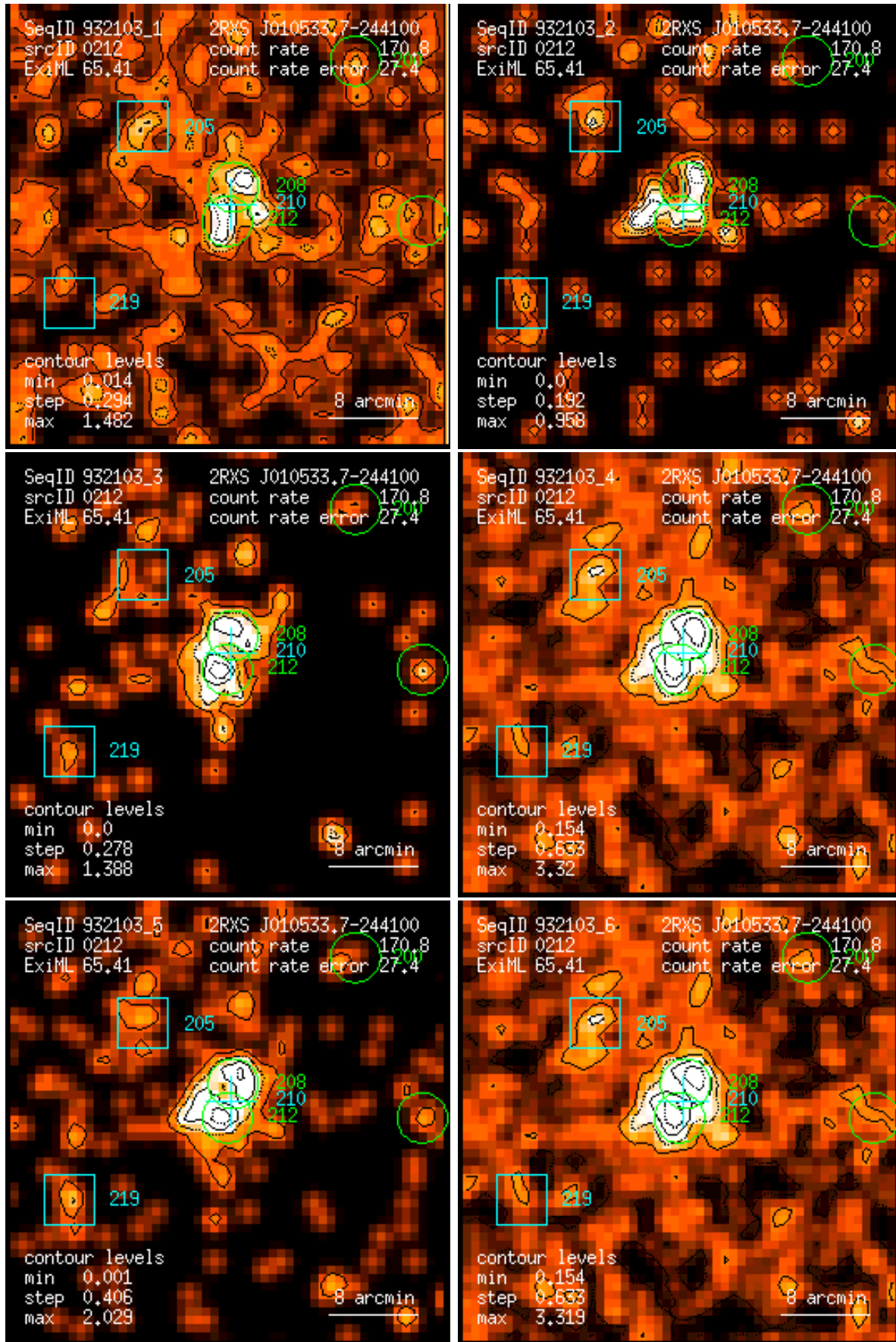
Figure 212: RASS 932103: detection 0212: band rate images, Gaussian filter: (1) PSPC channels 11 – 41, (2) 52 – 90, (3) 91 – 201, (4) 11 – 235, (5) 52 – 201, (6) 11 – 201. Broad band rates in counts/ks. Band rate contour levels in counts/ks/arcmin 2 .
