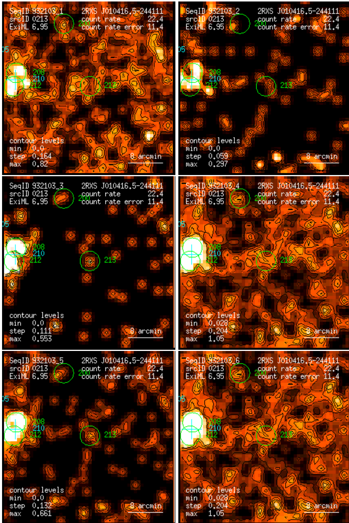
Figure 213: RASS 932103: detection 0213: band rate images, Gaussian filter: (1) PSPC channels 11 – 41, (2) 52 – 90, (3) 91 – 201, (4) 11 – 235, (5) 52 – 201, (6) 11 – 201. Broad band rates in counts/ks. Band rate contour levels in counts/ks/arcmin 2 .
