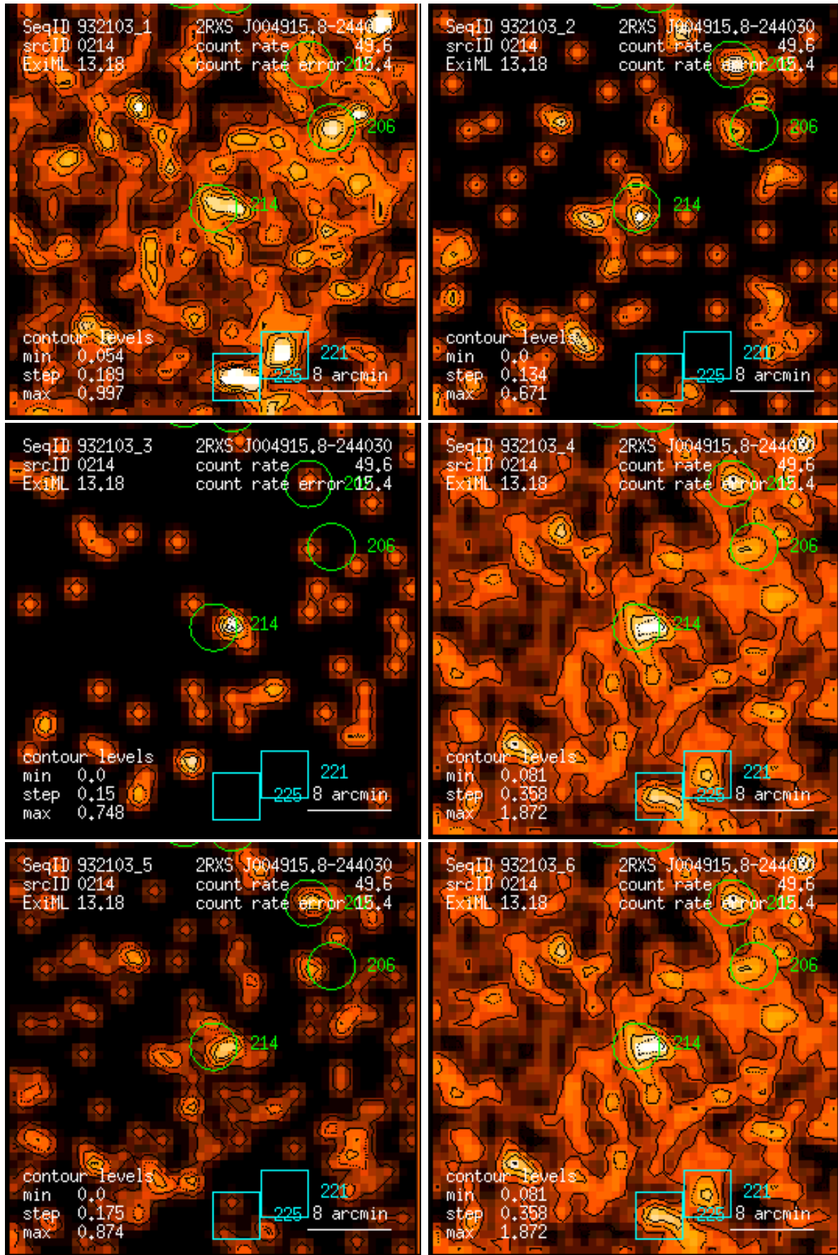
Figure 214: RASS 932103: detection 0214: band rate images, Gaussian filter: (1) PSPC channels 11 – 41, (2) 52 – 90, (3) 91 – 201, (4) 11 – 235, (5) 52 – 201, (6) 11 – 201. Broad band rates in counts/ks. Band rate contour levels in counts/ks/arcmin 2 .
