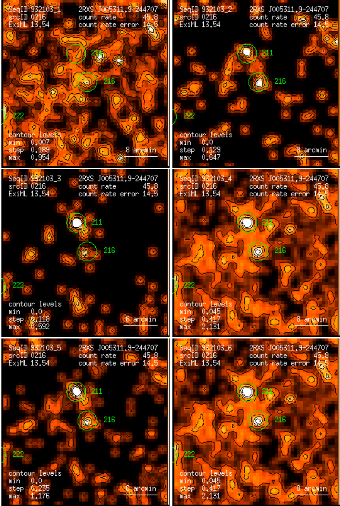
Figure 216: RASS 932103: detection 0216: band rate images, Gaussian filter: (1) PSPC channels 11 – 41, (2) 52 – 90, (3) 91 – 201, (4) 11 – 235, (5) 52 – 201, (6) 11 – 201. Broad band rates in counts/ks. Band rate contour levels in counts/ks/arcmin 2 .
