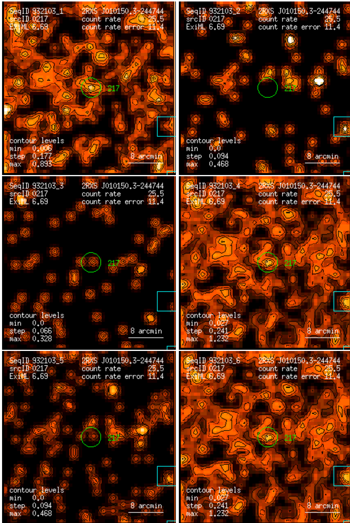
Figure 217: RASS 932103: detection 0217: band rate images, Gaussian filter: (1) PSPC channels 11 – 41, (2) 52 – 90, (3) 91 – 201, (4) 11 – 235, (5) 52 – 201, (6) 11 – 201. Broad band rates in counts/ks. Band rate contour levels in counts/ks/arcmin 2 .
