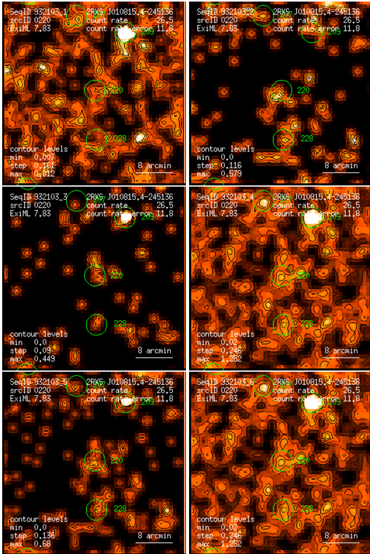
Figure 220: RASS 932103: detection 0220: band rate images, Gaussian filter: (1) PSPC channels 11 – 41, (2) 52 – 90, (3) 91 – 201, (4) 11 – 235, (5) 52 – 201, (6) 11 – 201. Broad band rates in counts/ks. Band rate contour levels in counts/ks/arcmin 2 .
