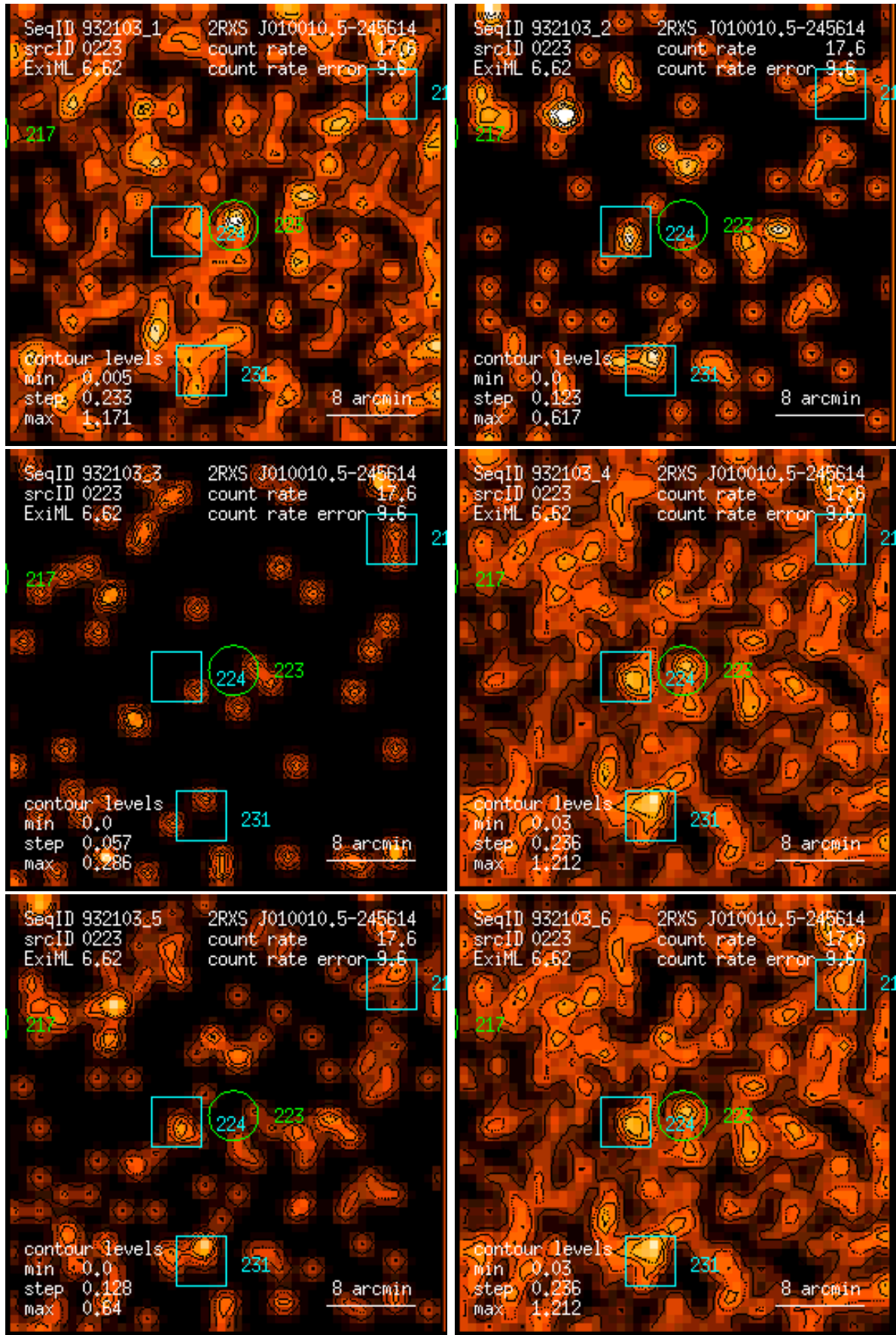
Figure 223: RASS 932103: detection 0223: band rate images, Gaussian filter: (1) PSPC channels 11 – 41, (2) 52 – 90, (3) 91 – 201, (4) 11 – 235, (5) 52 – 201, (6) 11 – 201. Broad band rates in counts/ks. Band rate contour levels in counts/ks/arcmin 2 .
