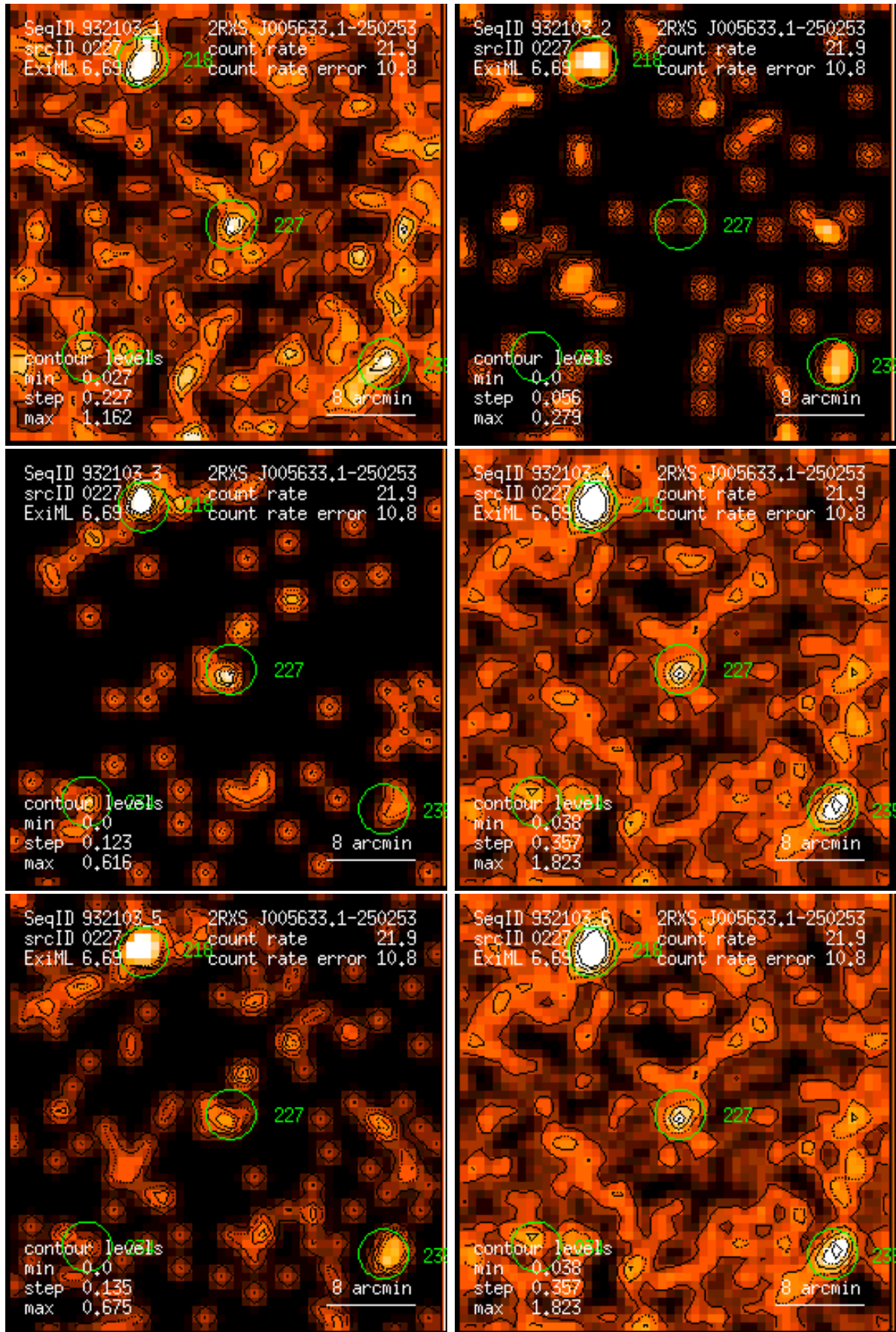
Figure 227: RASS 932103: detection 0227: band rate images, Gaussian filter: (1) PSPC channels 11 – 41, (2) 52 – 90, (3) 91 – 201, (4) 11 – 235, (5) 52 – 201, (6) 11 – 201. Broad band rates in counts/ks. Band rate contour levels in counts/ks/arcmin 2 .
