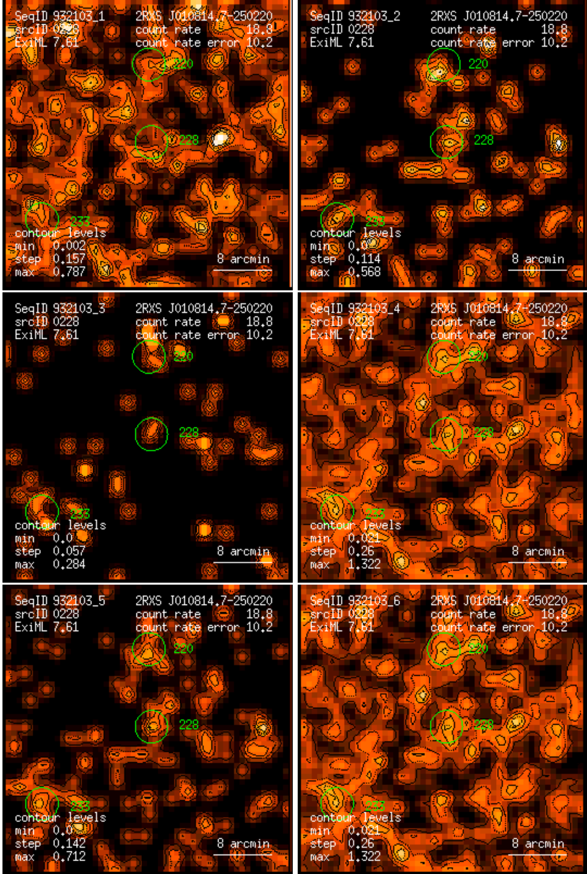
Figure 228: RASS 932103: detection 0228: band rate images, Gaussian filter: (1) PSPC channels 11 – 41, (2) 52 – 90, (3) 91 – 201, (4) 11 – 235, (5) 52 – 201, (6) 11 – 201. Broad band rates in counts/ks. Band rate contour levels in counts/ks/arcmin 2 .
