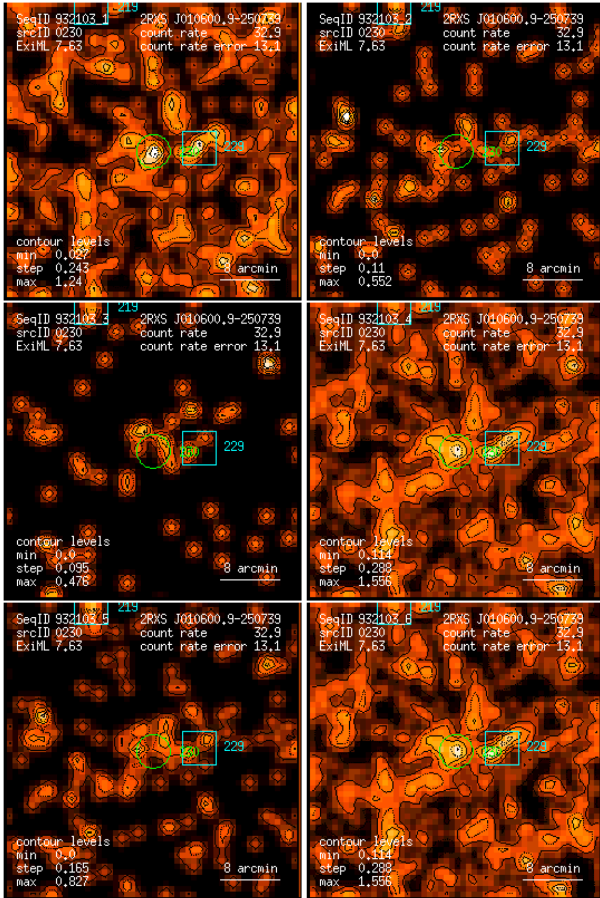
Figure 230: RASS 932103: detection 0230: band rate images, Gaussian filter: (1) PSPC channels 11 – 41, (2) 52 – 90, (3) 91 – 201, (4) 11 – 235, (5) 52 – 201, (6) 11 – 201. Broad band rates in counts/ks. Band rate contour levels in counts/ks/arcmin 2 .
