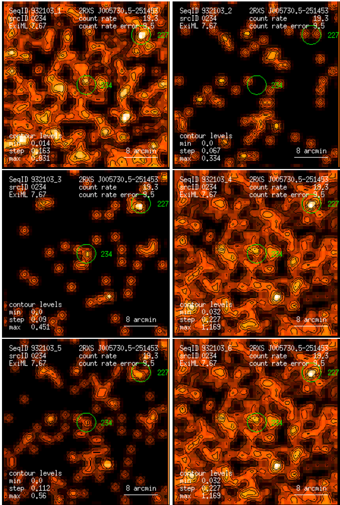
Figure 234: RASS 932103: detection 0234: band rate images, Gaussian filter: (1) PSPC channels 11 – 41, (2) 52 – 90, (3) 91 – 201, (4) 11 – 235, (5) 52 – 201, (6) 11 – 201. Broad band rates in counts/ks. Band rate contour levels in counts/ks/arcmin 2 .
