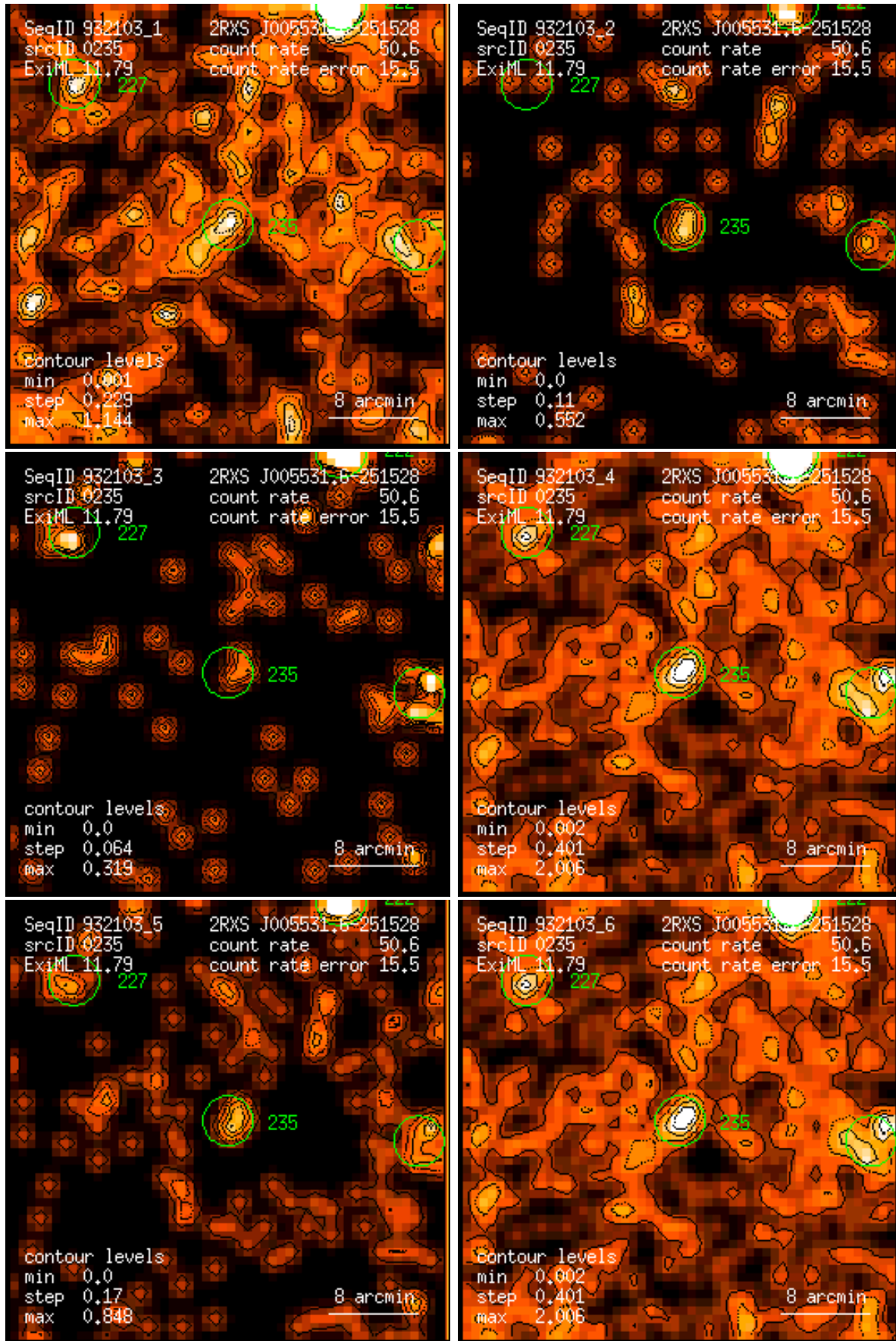
Figure 235: RASS 932103: detection 0235: band rate images, Gaussian filter: (1) PSPC channels 11 – 41, (2) 52 – 90, (3) 91 – 201, (4) 11 – 235, (5) 52 – 201, (6) 11 – 201. Broad band rates in counts/ks. Band rate contour levels in counts/ks/arcmin 2 .
