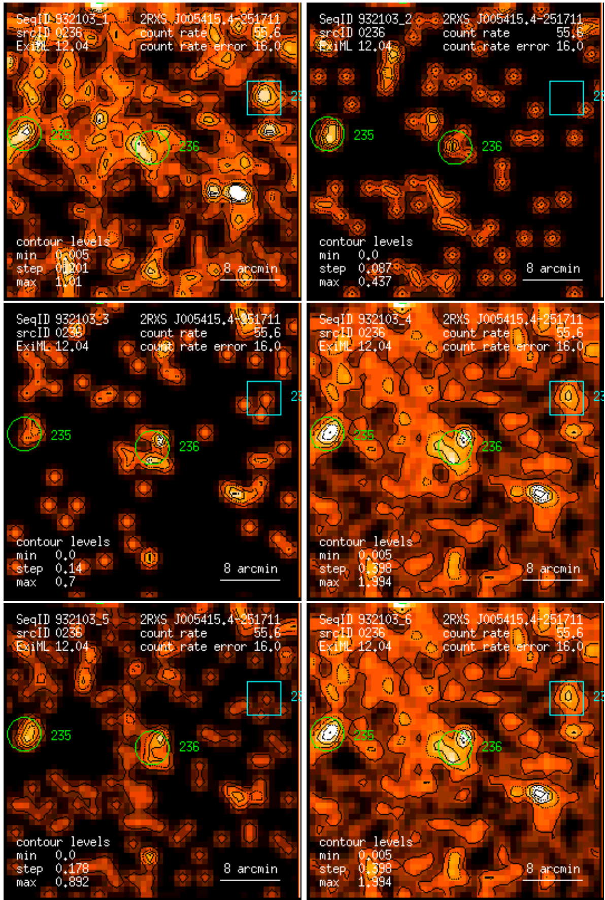
Figure 236: RASS 932103: detection 0236: band rate images, Gaussian filter: (1) PSPC channels 11 – 41, (2) 52 – 90, (3) 91 – 201, (4) 11 – 235, (5) 52 – 201, (6) 11 – 201. Broad band rates in counts/ks. Band rate contour levels in counts/ks/arcmin 2 .
