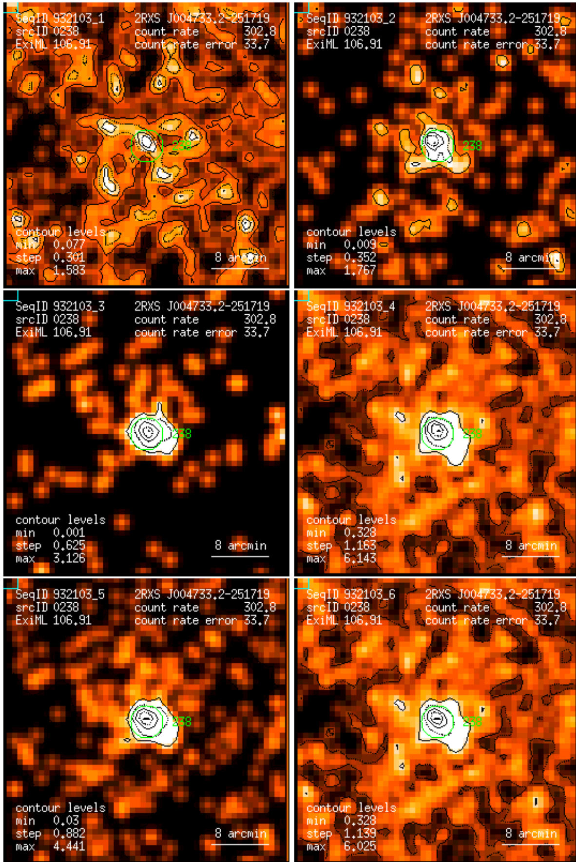
Figure 238: RASS 932103: detection 0238: band rate images, Gaussian filter: (1) PSPC channels 11 – 41, (2) 52 – 90, (3) 91 – 201, (4) 11 – 235, (5) 52 – 201, (6) 11 – 201. Broad band rates in counts/ks. Band rate contour levels in counts/ks/arcmin 2 .
