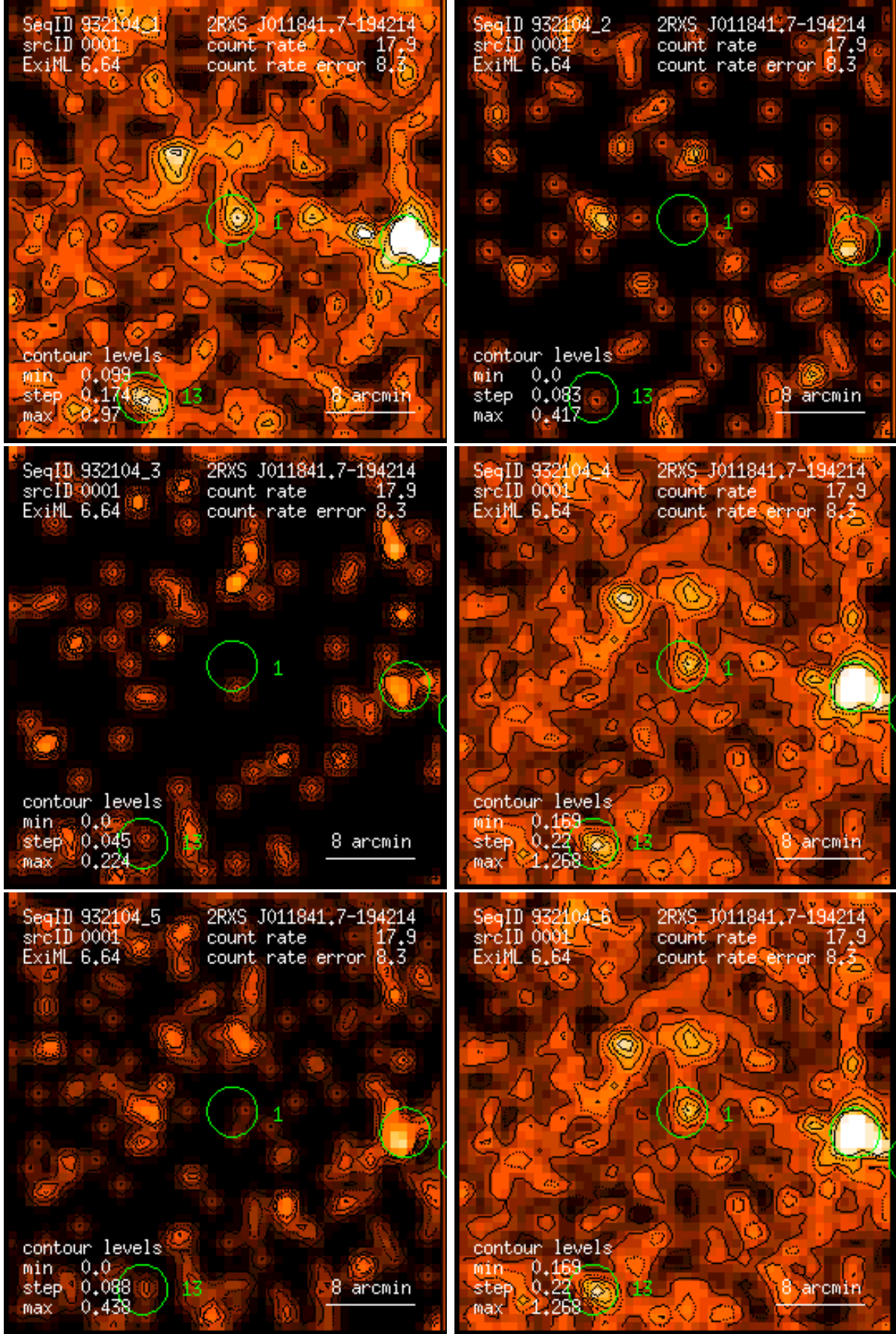
Figure 1: RASS 932104: detection 0001: band rate images, Gaussian filter: (1) PSPC channels 11 – 41, (2) 52 – 90, (3) 91 – 201, (4) 11 – 235, (5) 52 – 201, (6) 11 – 201. Broad band rates in counts/ks. Band rate contour levels in counts/ks/arcmin 2 .
