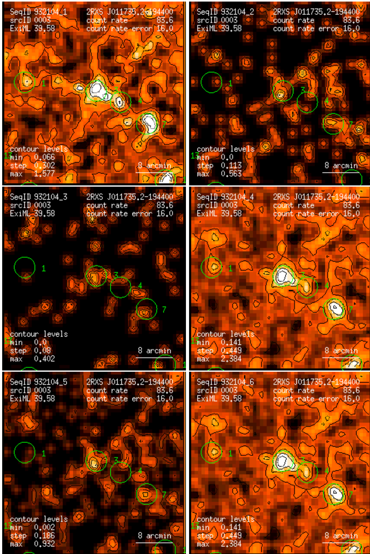
Figure 3: RASS 932104: detection 0003: band rate images, Gaussian filter: (1) PSPC channels 11 – 41, (2) 52 – 90, (3) 91 – 201, (4) 11 – 235, (5) 52 – 201, (6) 11 – 201. Broad band rates in counts/ks. Band rate contour levels in counts/ks/arcmin 2 .
