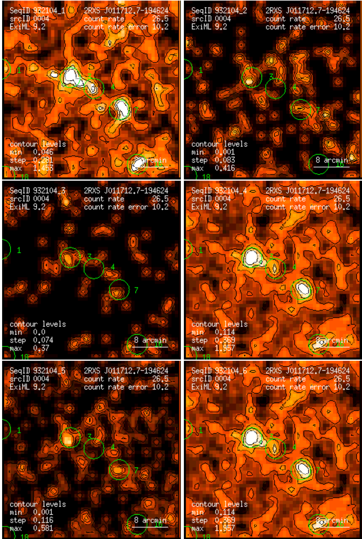
Figure 4: RASS 932104: detection 0004: band rate images, Gaussian filter: (1) PSPC channels 11 – 41, (2) 52 – 90, (3) 91 – 201, (4) 11 – 235, (5) 52 – 201, (6) 11 – 201. Broad band rates in counts/ks. Band rate contour levels in counts/ks/arcmin 2 .
