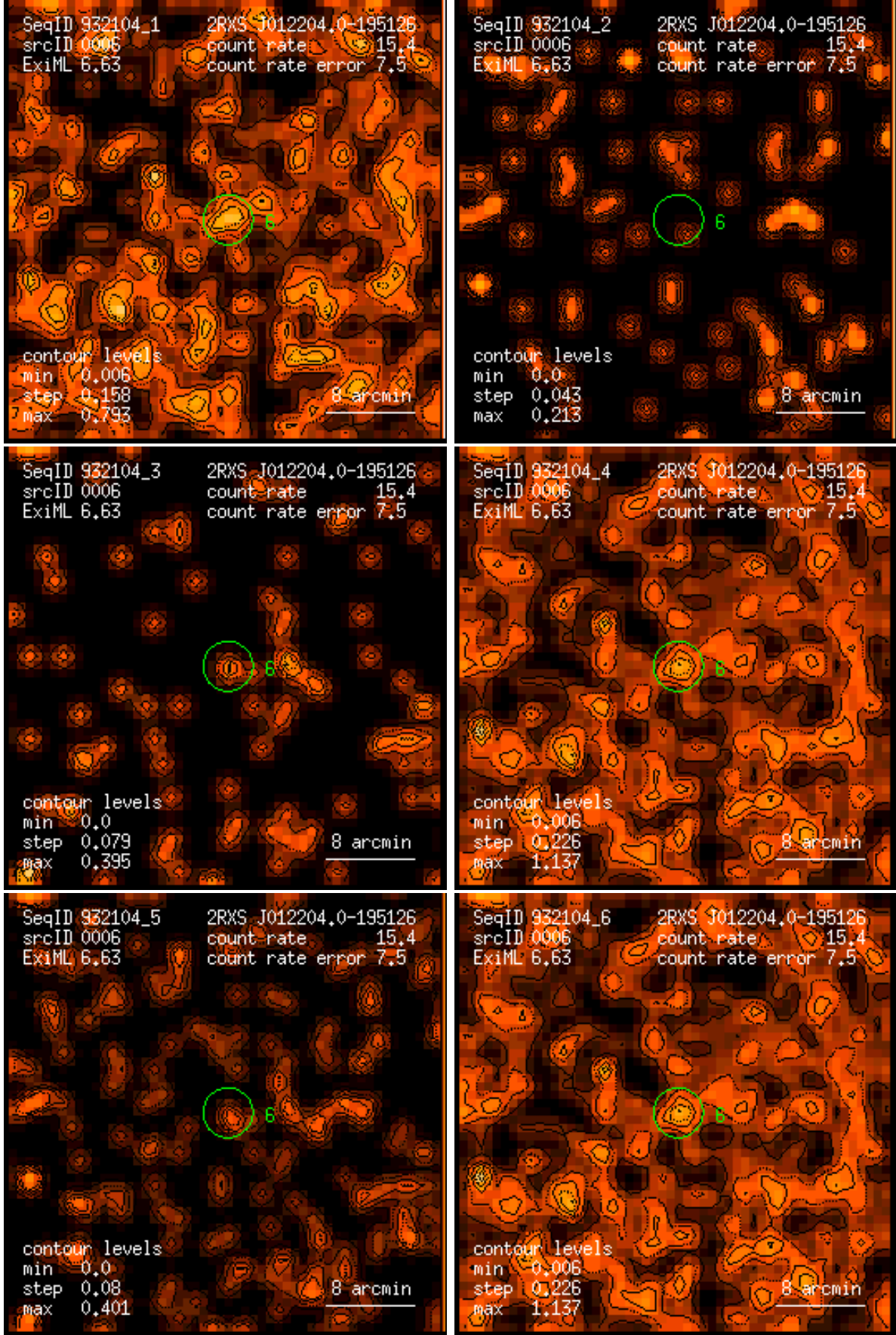
Figure 6: RASS 932104: detection 0006: band rate images, Gaussian filter: (1) PSPC channels 11 – 41, (2) 52 – 90, (3) 91 – 201, (4) 11 – 235, (5) 52 – 201, (6) 11 – 201. Broad band rates in counts/ks. Band rate contour levels in counts/ks/arcmin 2 .
