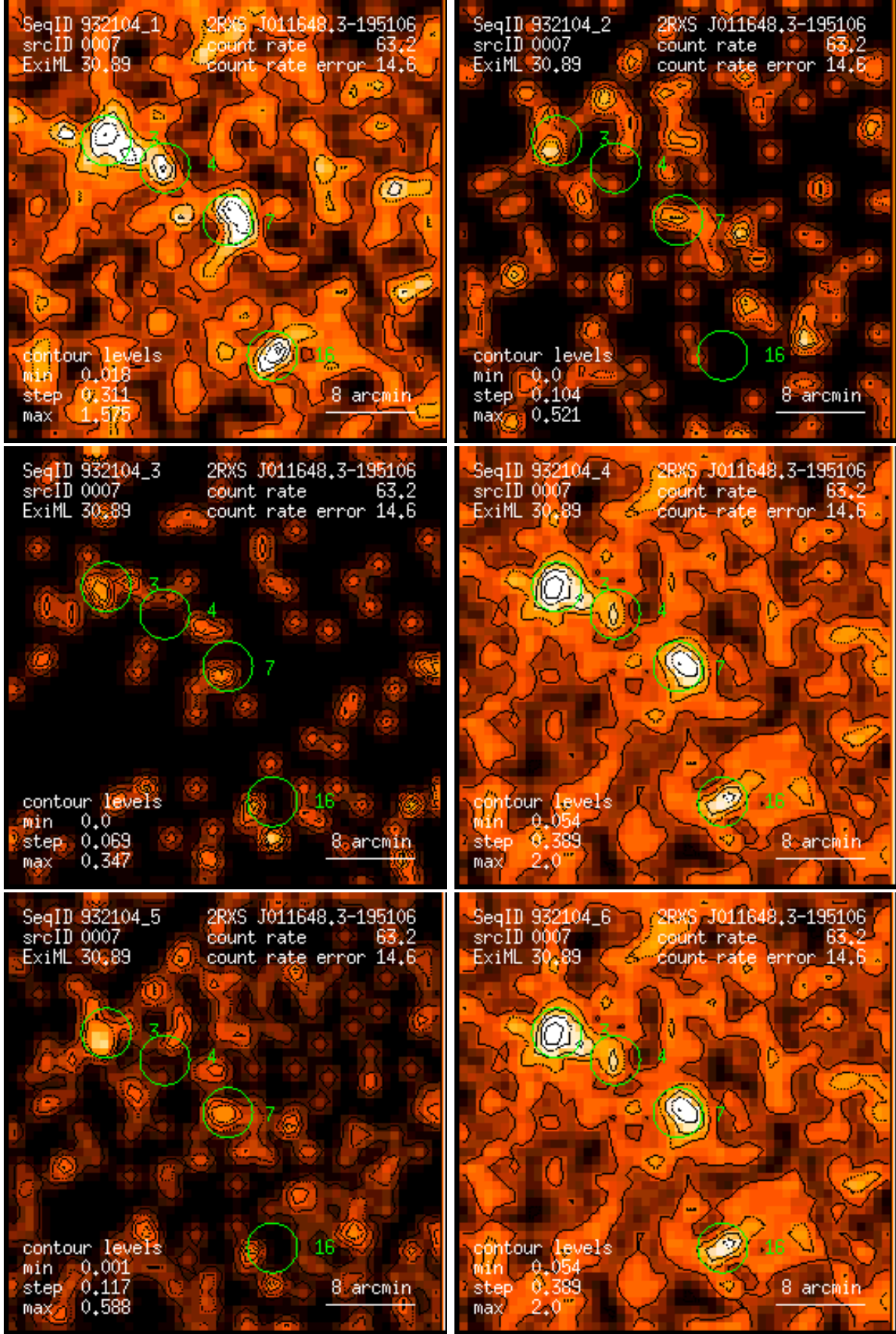
Figure 7: RASS 932104: detection 0007: band rate images, Gaussian filter: (1) PSPC channels 11 – 41, (2) 52 – 90, (3) 91 – 201, (4) 11 – 235, (5) 52 – 201, (6) 11 – 201. Broad band rates in counts/ks. Band rate contour levels in counts/ks/arcmin 2 .
