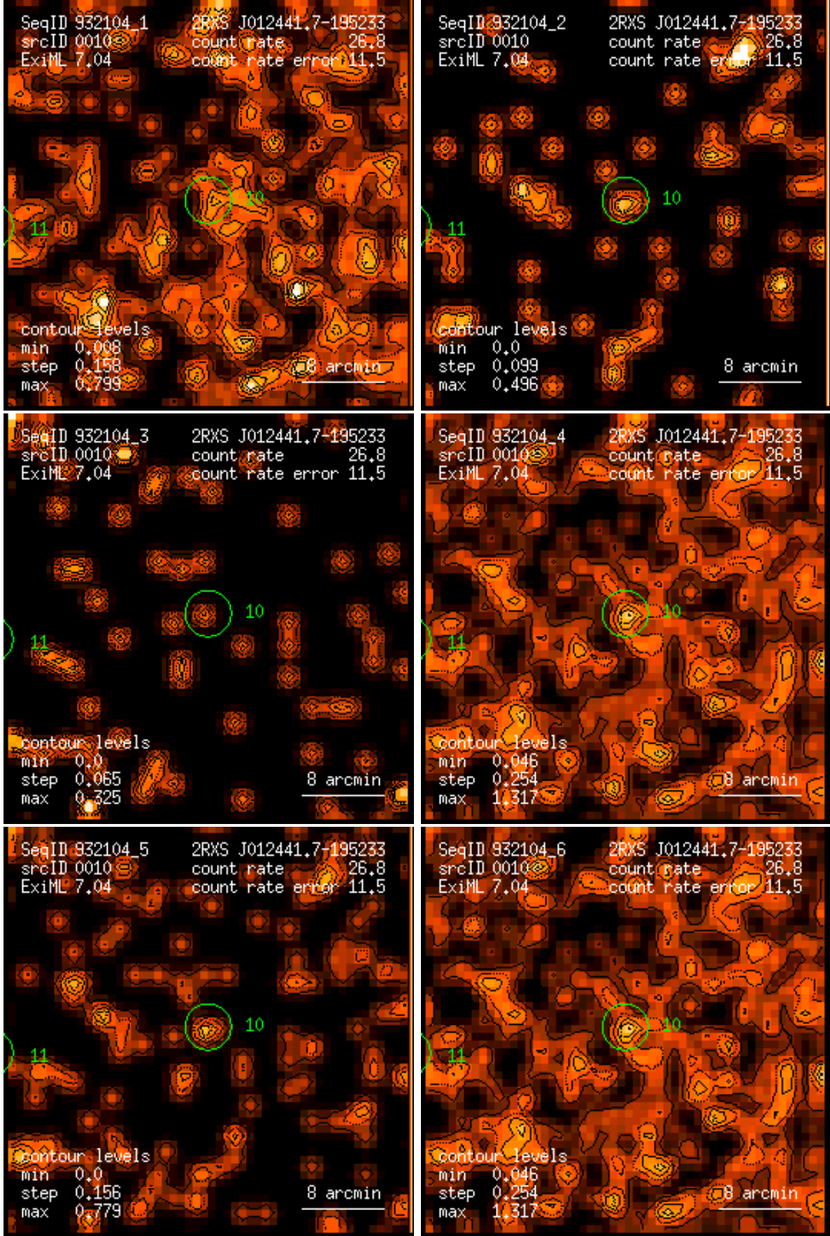
Figure 10: RASS 932104: detection 0010: band rate images, Gaussian filter: (1) PSPC channels 11 – 41, (2) 52 – 90, (3) 91 – 201, (4) 11 – 235, (5) 52 – 201, (6) 11 – 201. Broad band rates in counts/ks. Band rate contour levels in counts/ks/arcmin 2 .
