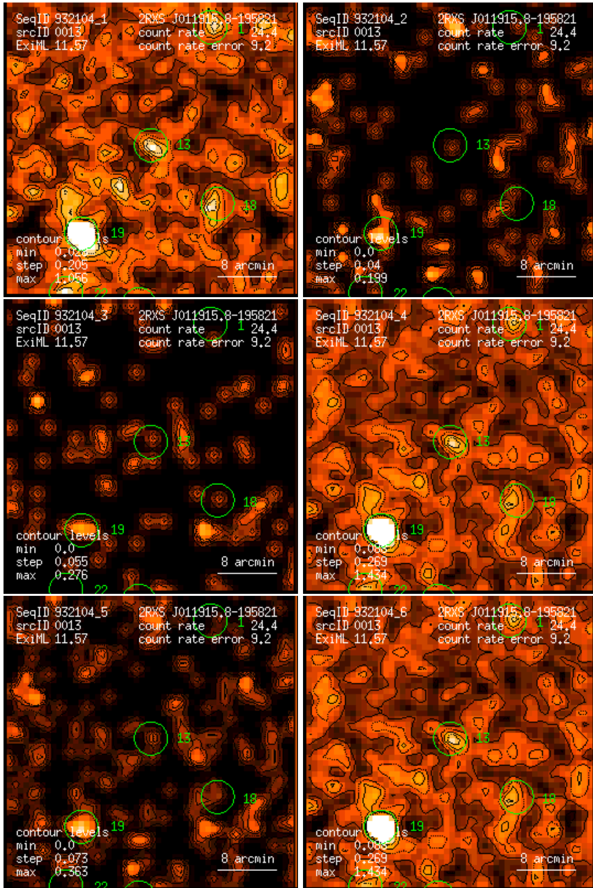
Figure 13: RASS 932104: detection 0013: band rate images, Gaussian filter: (1) PSPC channels 11 – 41, (2) 52 – 90, (3) 91 – 201, (4) 11 – 235, (5) 52 – 201, (6) 11 – 201. Broad band rates in counts/ks. Band rate contour levels in counts/ks/arcmin 2 .
