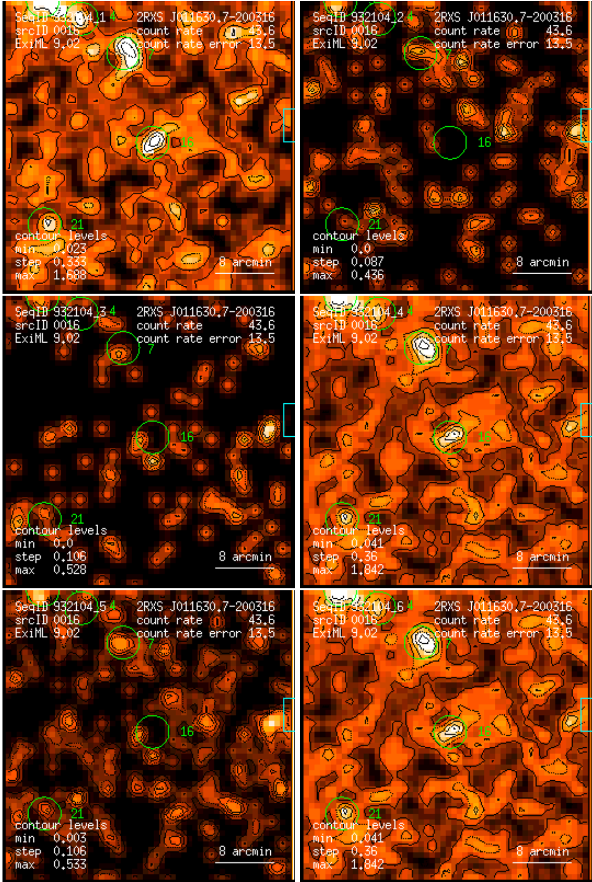
Figure 16: RASS 932104: detection 0016: band rate images, Gaussian filter: (1) PSPC channels 11 – 41, (2) 52 – 90, (3) 91 – 201, (4) 11 – 235, (5) 52 – 201, (6) 11 – 201. Broad band rates in counts/ks. Band rate contour levels in counts/ks/arcmin 2 .
