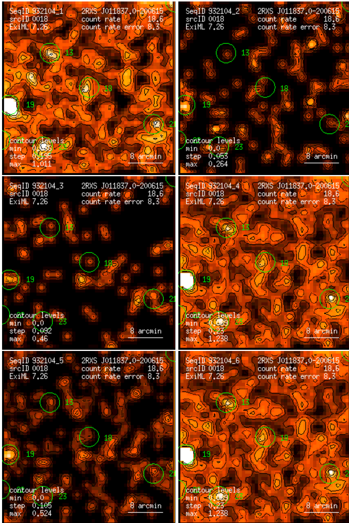
Figure 18: RASS 932104: detection 0018: band rate images, Gaussian filter: (1) PSPC channels 11 – 41, (2) 52 – 90, (3) 91 – 201, (4) 11 – 235, (5) 52 – 201, (6) 11 – 201. Broad band rates in counts/ks. Band rate contour levels in counts/ks/arcmin 2 .
