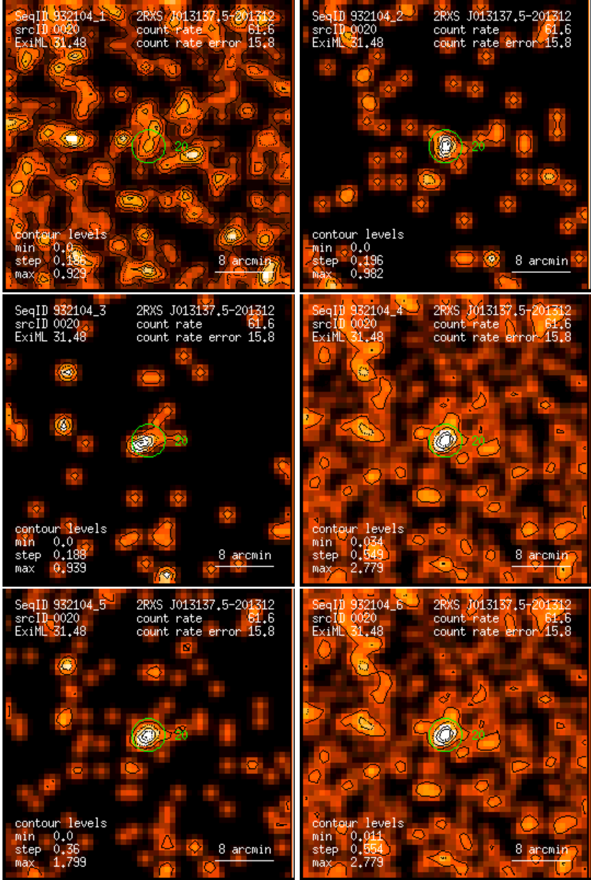
Figure 20: RASS 932104: detection 0020: band rate images, Gaussian filter: (1) PSPC channels 11 – 41, (2) 52 – 90, (3) 91 – 201, (4) 11 – 235, (5) 52 – 201, (6) 11 – 201. Broad band rates in counts/ks. Band rate contour levels in counts/ks/arcmin 2 .
