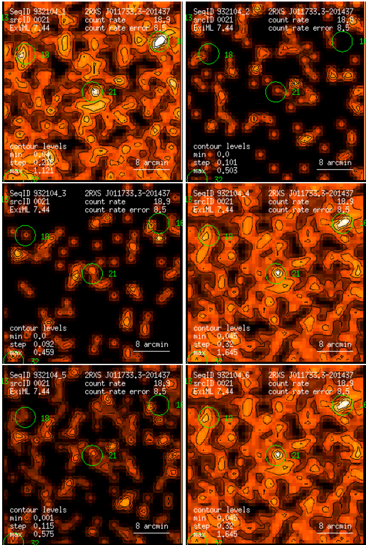
Figure 21: RASS 932104: detection 0021: band rate images, Gaussian filter: (1) PSPC channels 11 – 41, (2) 52 – 90, (3) 91 – 201, (4) 11 – 235, (5) 52 – 201, (6) 11 – 201. Broad band rates in counts/ks. Band rate contour levels in counts/ks/arcmin 2 .
