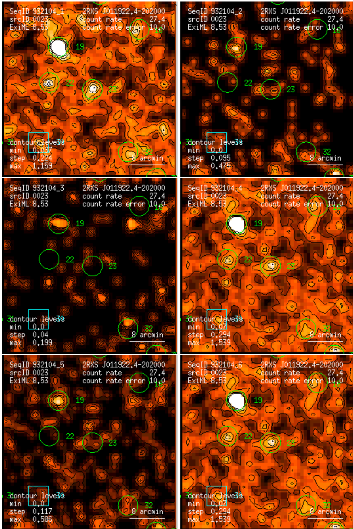
Figure 23: RASS 932104: detection 0023: band rate images, Gaussian filter: (1) PSPC channels 11 – 41, (2) 52 – 90, (3) 91 – 201, (4) 11 – 235, (5) 52 – 201, (6) 11 – 201. Broad band rates in counts/ks. Band rate contour levels in counts/ks/arcmin 2 .
