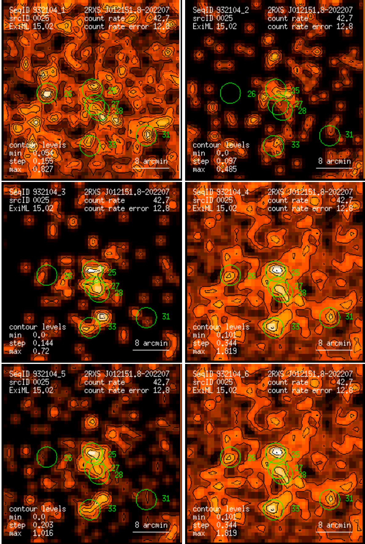
Figure 25: RASS 932104: detection 0025: band rate images, Gaussian filter: (1) PSPC channels 11 – 41, (2) 52 – 90, (3) 91 – 201, (4) 11 – 235, (5) 52 – 201, (6) 11 – 201. Broad band rates in counts/ks. Band rate contour levels in counts/ks/arcmin 2 .
