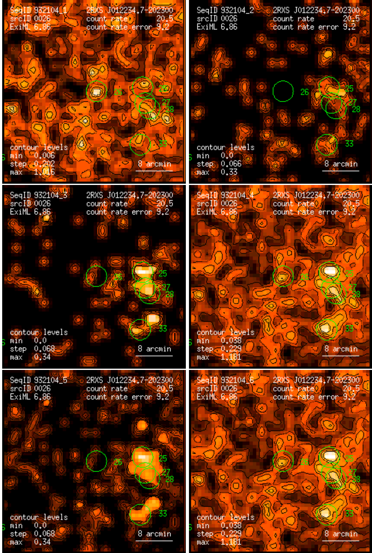
Figure 26: RASS 932104: detection 0026: band rate images, Gaussian filter: (1) PSPC channels 11 – 41, (2) 52 – 90, (3) 91 – 201, (4) 11 – 235, (5) 52 – 201, (6) 11 – 201. Broad band rates in counts/ks. Band rate contour levels in counts/ks/arcmin 2 .
