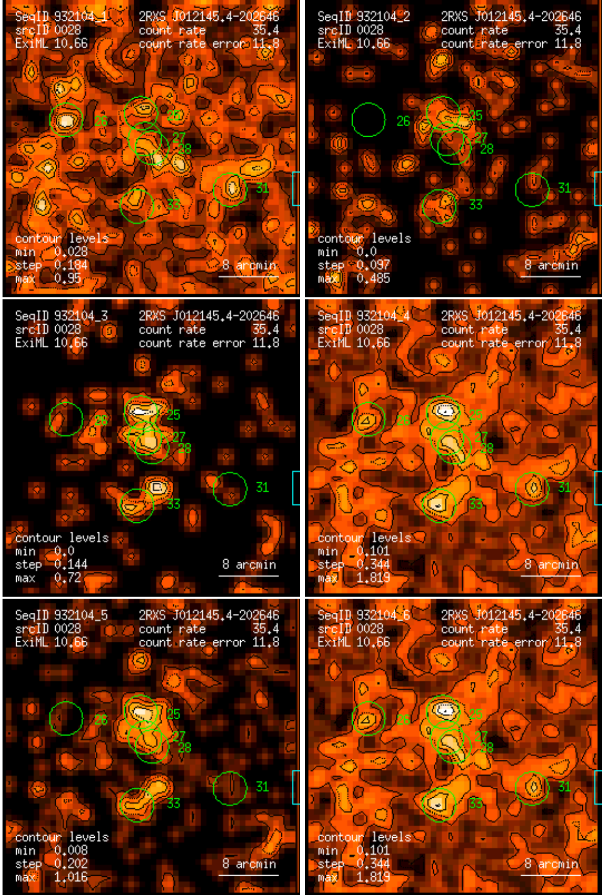
Figure 28: RASS 932104: detection 0028: band rate images, Gaussian filter: (1) PSPC channels 11 – 41, (2) 52 – 90, (3) 91 – 201, (4) 11 – 235, (5) 52 – 201, (6) 11 – 201. Broad band rates in counts/ks. Band rate contour levels in counts/ks/arcmin 2 .
