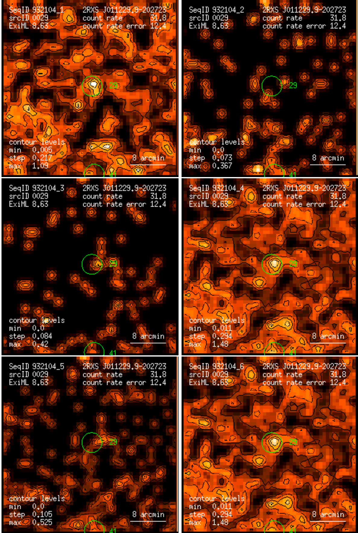
Figure 29: RASS 932104: detection 0029: band rate images, Gaussian filter: (1) PSPC channels 11 – 41, (2) 52 – 90, (3) 91 – 201, (4) 11 – 235, (5) 52 – 201, (6) 11 – 201. Broad band rates in counts/ks. Band rate contour levels in counts/ks/arcmin 2 .
