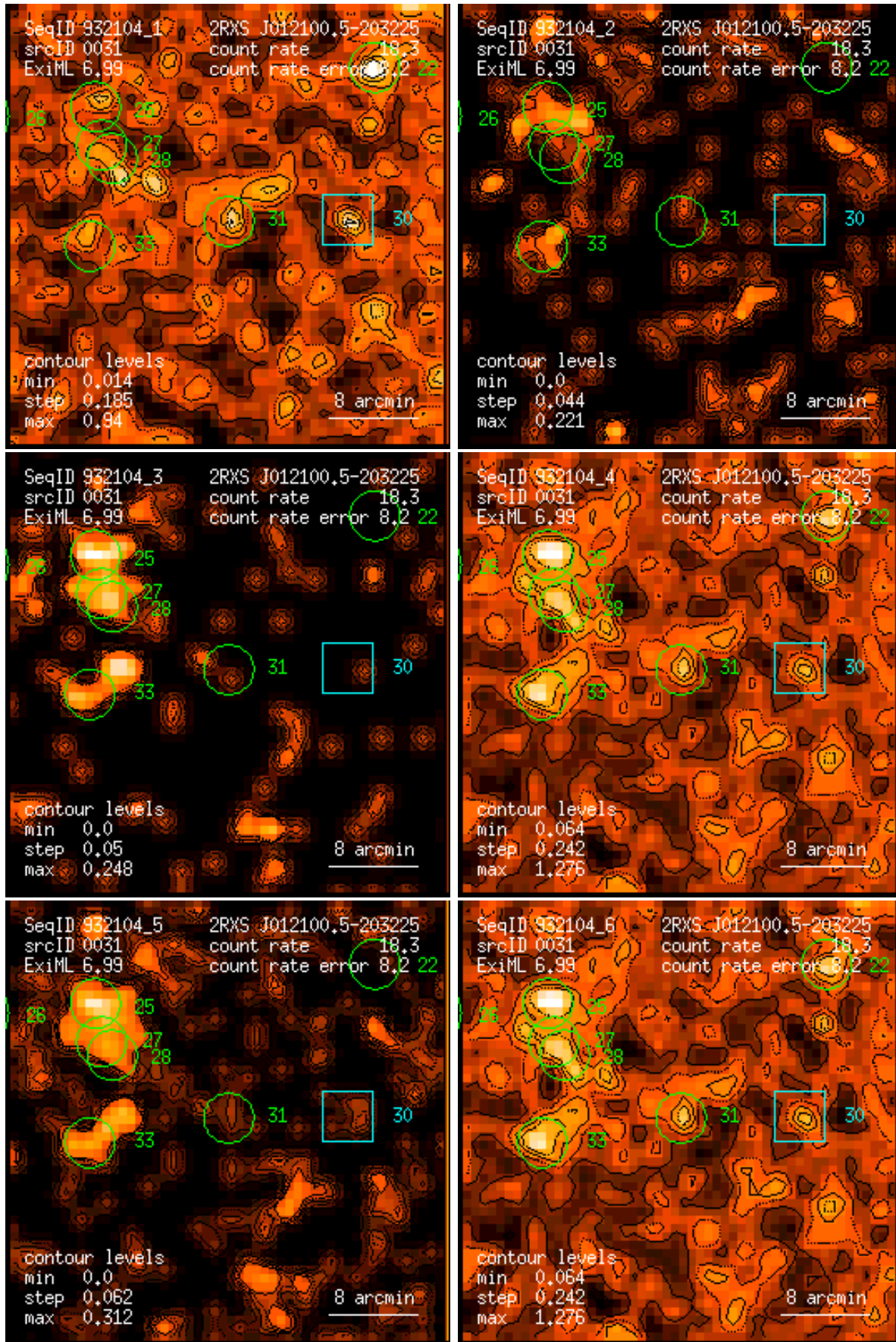
Figure 31: RASS 932104: detection 0031: band rate images, Gaussian filter: (1) PSPC channels 11 – 41, (2) 52 – 90, (3) 91 – 201, (4) 11 – 235, (5) 52 – 201, (6) 11 – 201. Broad band rates in counts/ks. Band rate contour levels in counts/ks/arcmin 2 .
