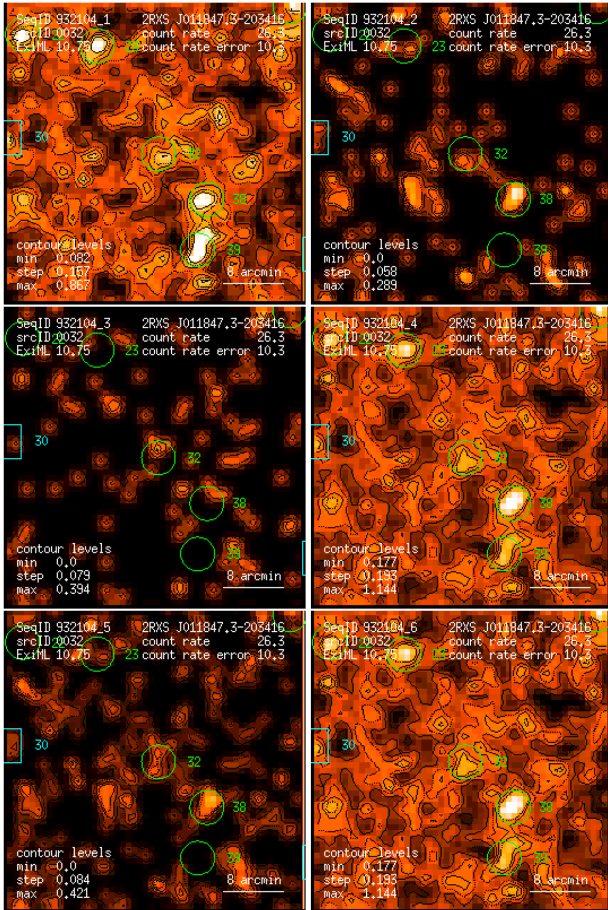
Figure 32: RASS 932104: detection 0032: band rate images, Gaussian filter: (1) PSPC channels 11 – 41, (2) 52 – 90, (3) 91 – 201, (4) 11 – 235, (5) 52 – 201, (6) 11 – 201. Broad band rates in counts/ks. Band rate contour levels in counts/ks/arcmin 2 .
