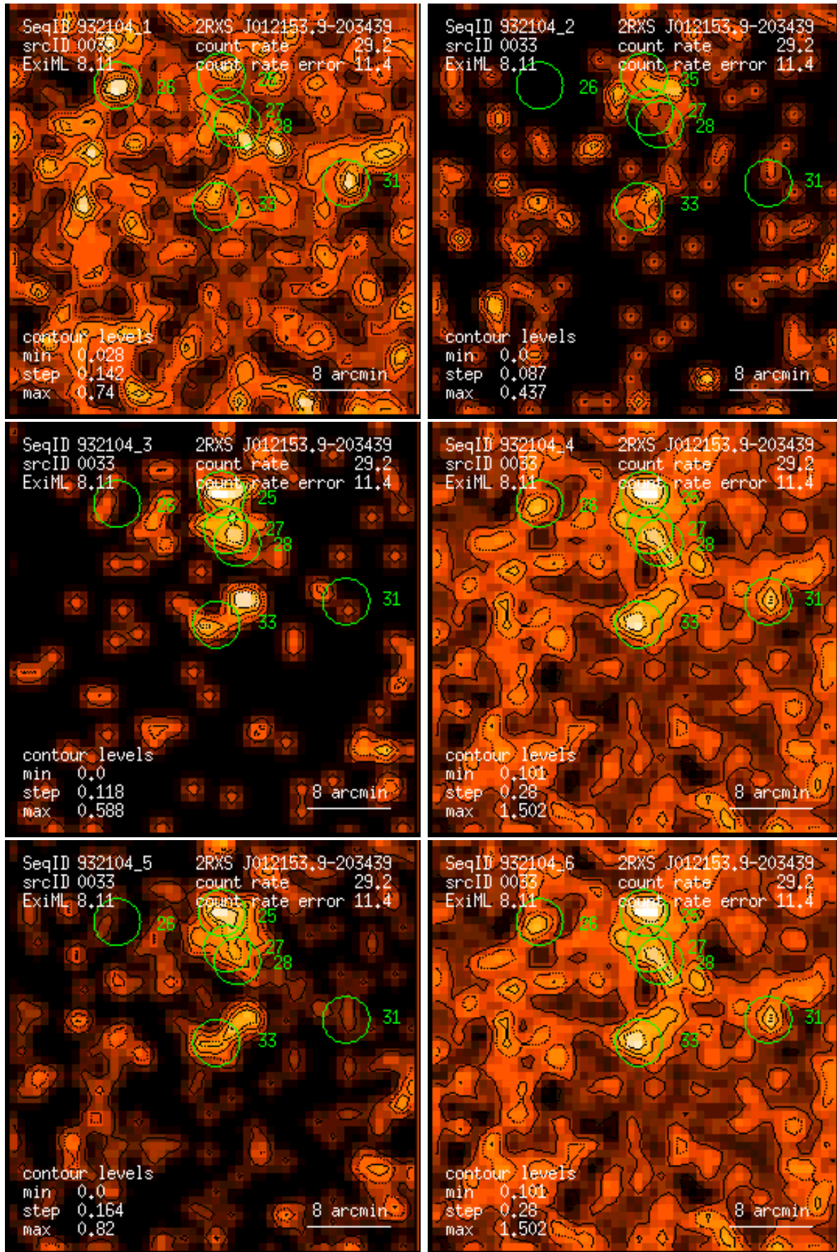
Figure 33: RASS 932104: detection 0033: band rate images, Gaussian filter: (1) PSPC channels 11 – 41, (2) 52 – 90, (3) 91 – 201, (4) 11 – 235, (5) 52 – 201, (6) 11 – 201. Broad band rates in counts/ks. Band rate contour levels in counts/ks/arcmin 2 .
