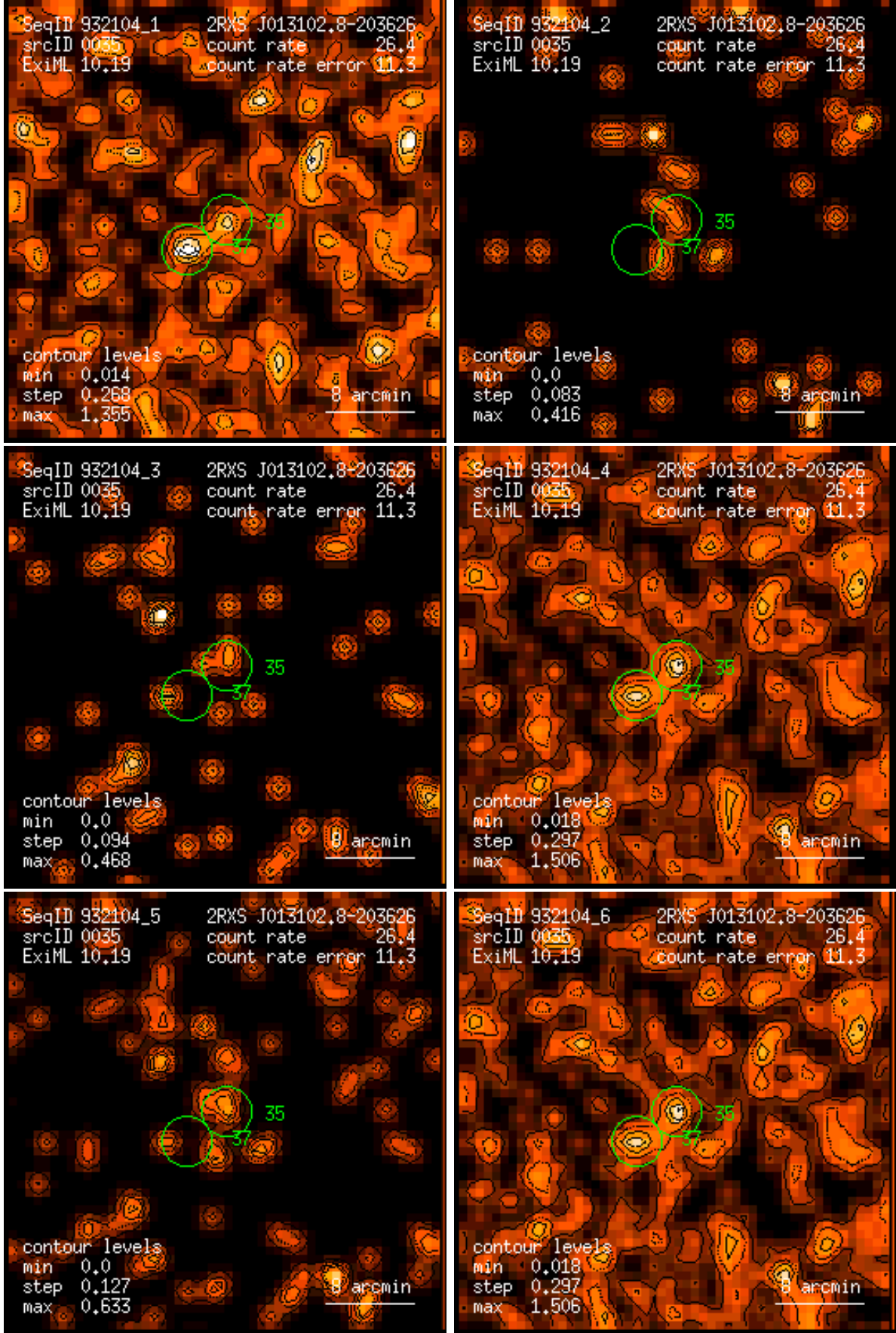
Figure 35: RASS 932104: detection 0035: band rate images, Gaussian filter: (1) PSPC channels 11 – 41, (2) 52 – 90, (3) 91 – 201, (4) 11 – 235, (5) 52 – 201, (6) 11 – 201. Broad band rates in counts/ks. Band rate contour levels in counts/ks/arcmin 2 .
