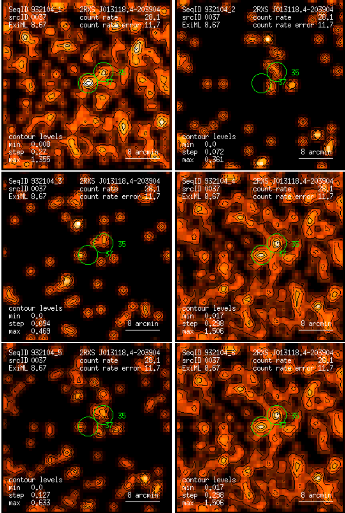
Figure 37: RASS 932104: detection 0037: band rate images, Gaussian filter: (1) PSPC channels 11 – 41, (2) 52 – 90, (3) 91 – 201, (4) 11 – 235, (5) 52 – 201, (6) 11 – 201. Broad band rates in counts/ks. Band rate contour levels in counts/ks/arcmin 2 .
