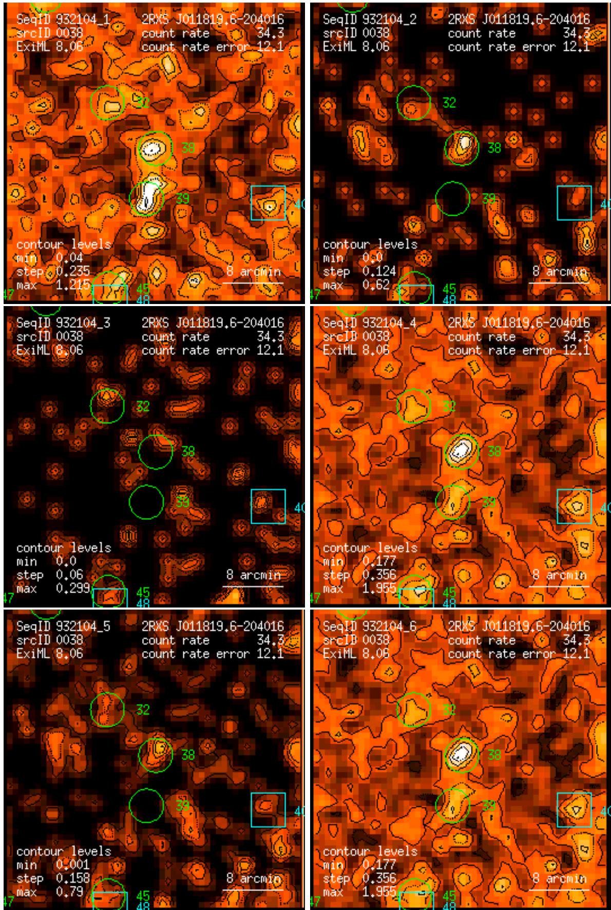
Figure 38: RASS 932104: detection 0038: band rate images, Gaussian filter: (1) PSPC channels 11 – 41, (2) 52 – 90, (3) 91 – 201, (4) 11 – 235, (5) 52 – 201, (6) 11 – 201. Broad band rates in counts/ks. Band rate contour levels in counts/ks/arcmin 2 .
