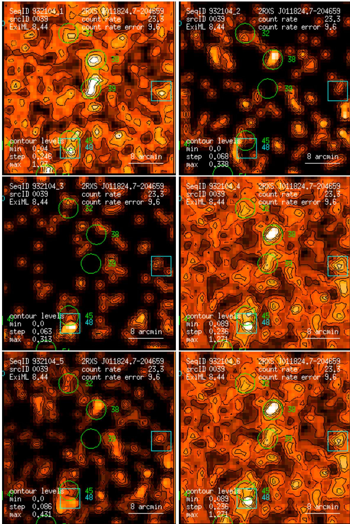
Figure 39: RASS 932104: detection 0039: band rate images, Gaussian filter: (1) PSPC channels 11 – 41, (2) 52 – 90, (3) 91 – 201, (4) 11 – 235, (5) 52 – 201, (6) 11 – 201. Broad band rates in counts/ks. Band rate contour levels in counts/ks/arcmin 2 .
