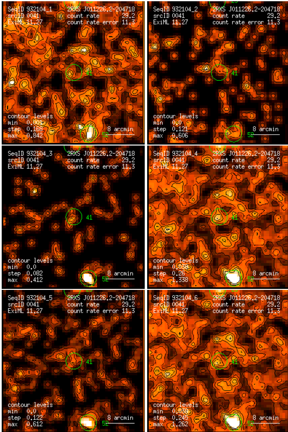
Figure 41: RASS 932104: detection 0041: band rate images, Gaussian filter: (1) PSPC channels 11 – 41, (2) 52 – 90, (3) 91 – 201, (4) 11 – 235, (5) 52 – 201, (6) 11 – 201. Broad band rates in counts/ks. Band rate contour levels in counts/ks/arcmin 2 .
