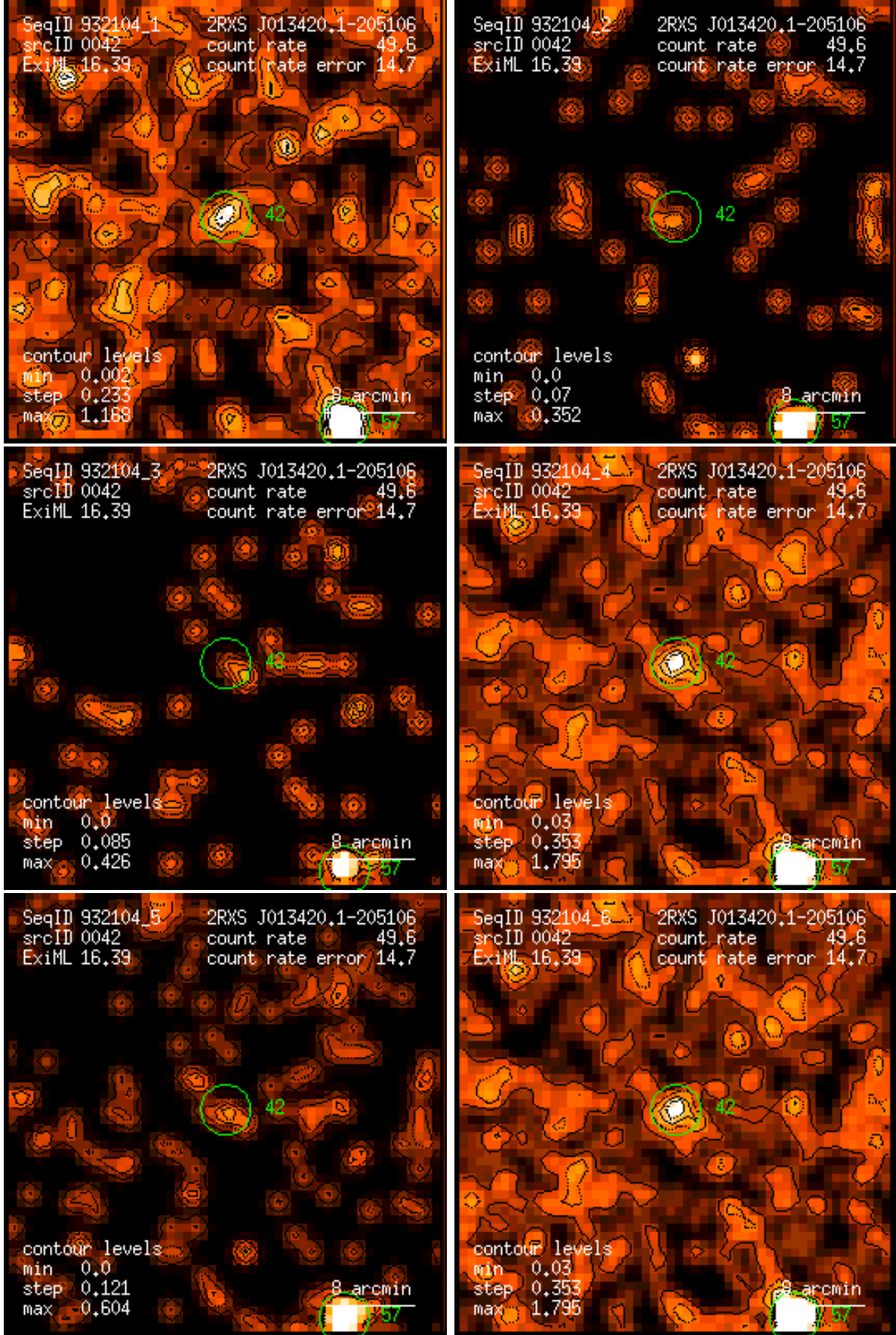
Figure 42: RASS 932104: detection 0042: band rate images, Gaussian filter: (1) PSPPC channels 11 – 41, (2) 52 – 90, (3) 91 – 201, (4) 11 – 235, (5) 52 – 201, (6) 11 – 201. Broad band rates in counts/ks. Band rate contour levels in counts/ks/arcmin 2 .
