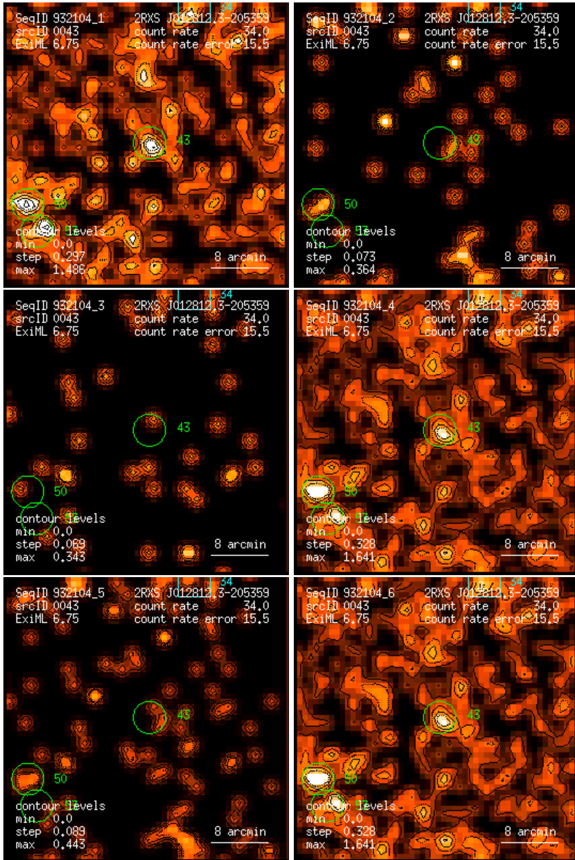
Figure 43: RASS 932104: detection 0043: band rate images, Gaussian filter: (1) PSPC channels 11 – 41, (2) 52 – 90, (3) 91 – 201, (4) 11 – 235, (5) 52 – 201, (6) 11 – 201. Broad band rates in counts/ks. Band rate contour levels in counts/ks/arcmin 2 .
