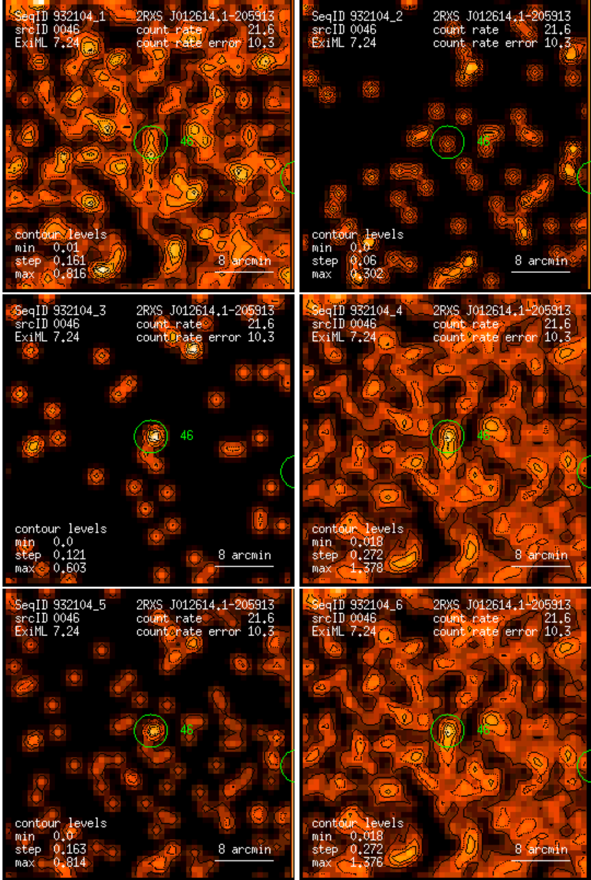
Figure 46: RASS 932104: detection 0046: band rate images, Gaussian filter: (1) PSPC channels 11 – 41, (2) 52 – 90, (3) 91 – 201, (4) 11 – 235, (5) 52 – 201, (6) 11 – 201. Broad band rates in counts/ks. Band rate contour levels in counts/ks/arcmin 2 .
