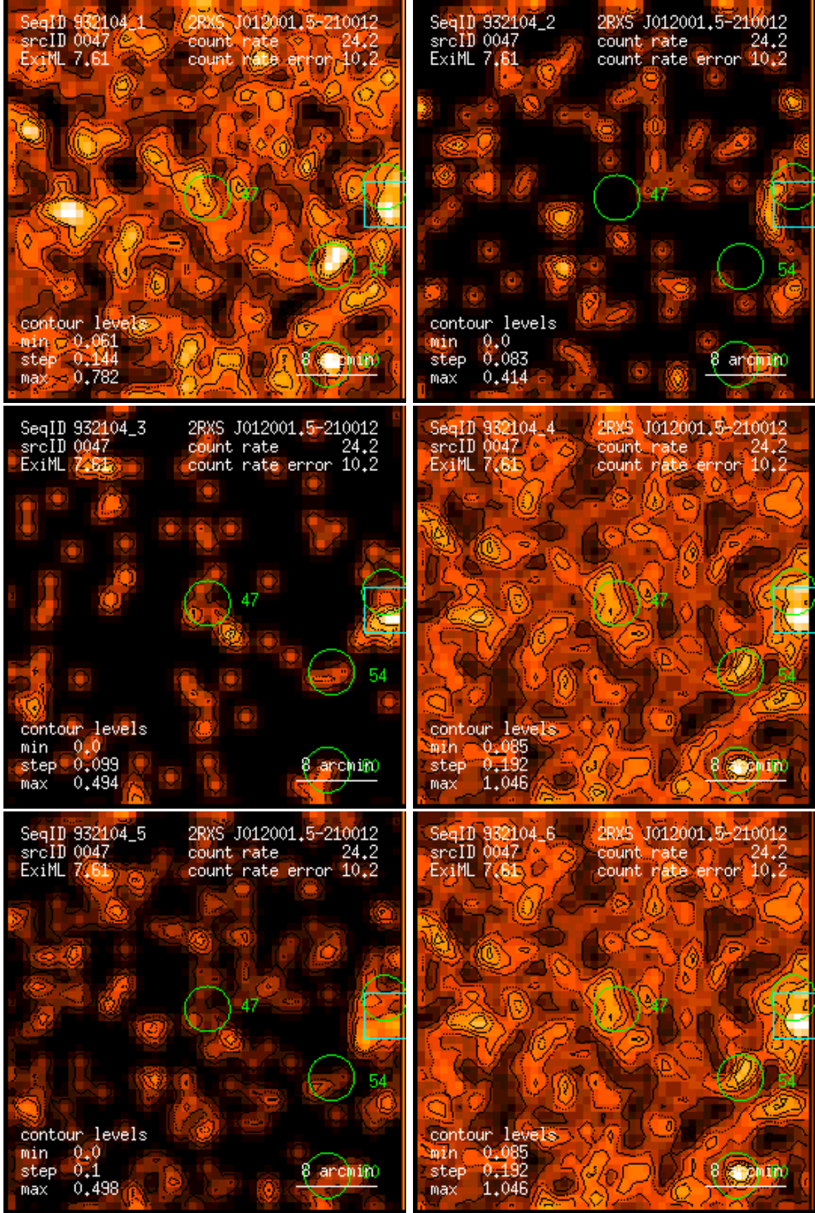
Figure 47: RASS 932104: detection 0047: band rate images, Gaussian filter: (1) PSPC channels 11 – 41, (2) 52 – 90, (3) 91 – 201, (4) 11 – 235, (5) 52 – 201, (6) 11 – 201. Broad band rates in counts/ks. Band rate contour levels in counts/ks/arcmin 2 .
