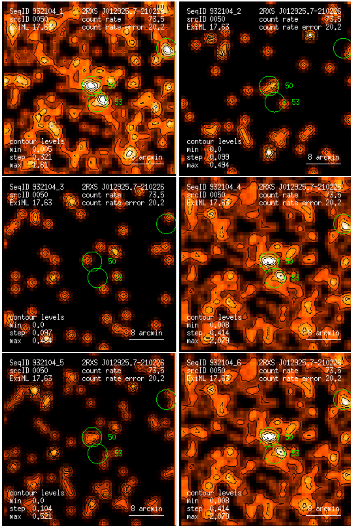
Figure 50: RASS 932104: detection 0050: band rate images, Gaussian filter: (1) PSPC channels 11 – 41, (2) 52 – 90, (3) 91 – 201, (4) 11 – 235, (5) 52 – 201, (6) 11 – 201. Broad band rates in counts/ks. Band rate contour levels in counts/ks/arcmin 2 .
