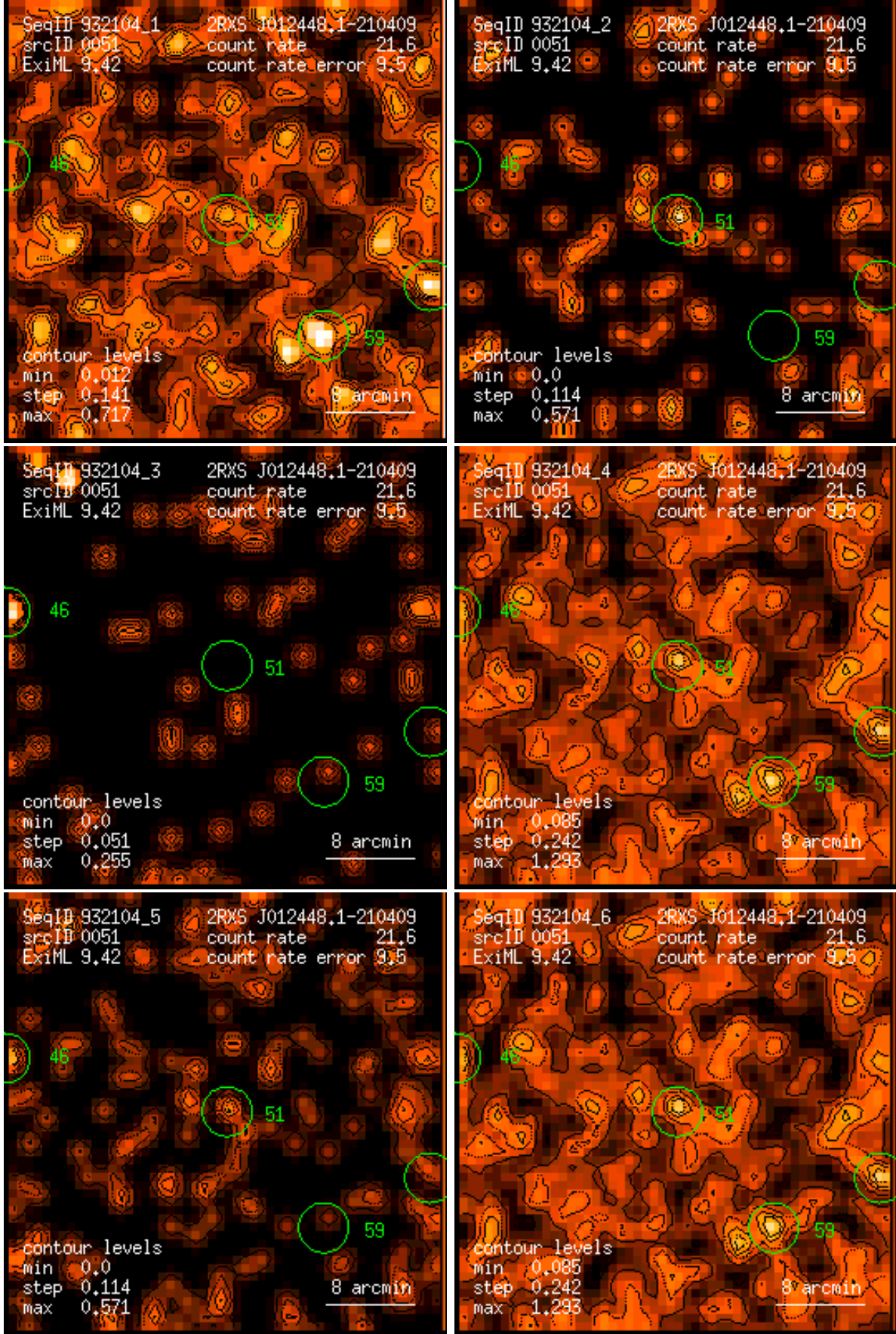
Figure 51: RASS 932104: detection 0051: band rate images, Gaussian filter: (1) PSPC channels 11 – 41, (2) 52 – 90, (3) 91 – 201, (4) 11 – 235, (5) 52 – 201, (6) 11 – 201. Broad band rates in counts/ks. Band rate contour levels in counts/ks/arcmin 2 .
