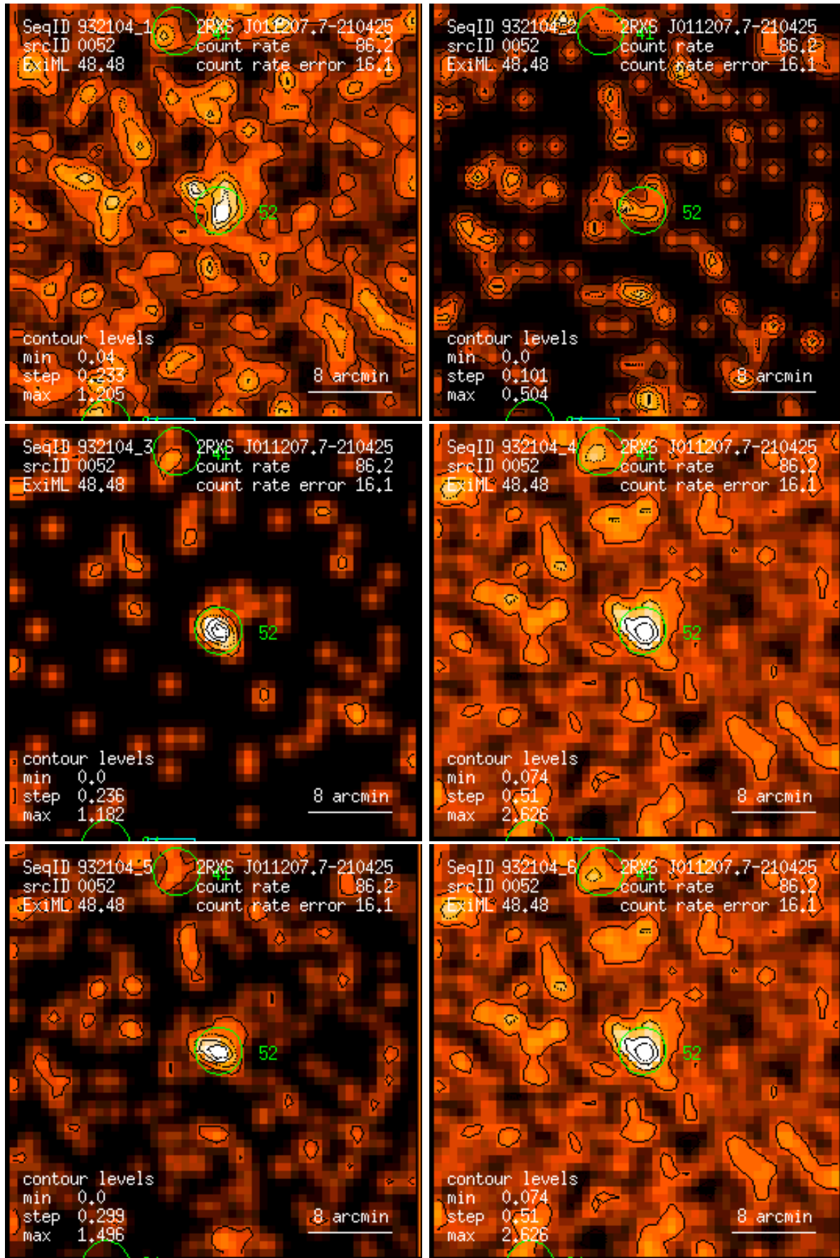
Figure 52: RASS 932104: detection 0052: band rate images, Gaussian filter: (1) PSPC channels 11 – 41, (2) 52 – 90, (3) 91 – 201, (4) 11 – 235, (5) 52 – 201, (6) 11 – 201. Broad band rates in counts/ks. Band rate contour levels in counts/ks/arcmin 2 .
