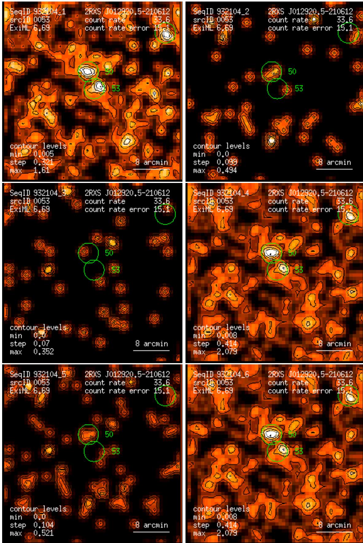
Figure 53: RASS 932104: detection 0053: band rate images, Gaussian filter: (1) PSPC channels 11 – 41, (2) 52 – 90, (3) 91 – 201, (4) 11 – 235, (5) 52 – 201, (6) 11 – 201. Broad band rates in counts/ks. Band rate contour levels in counts/ks/arcmin 2 .
