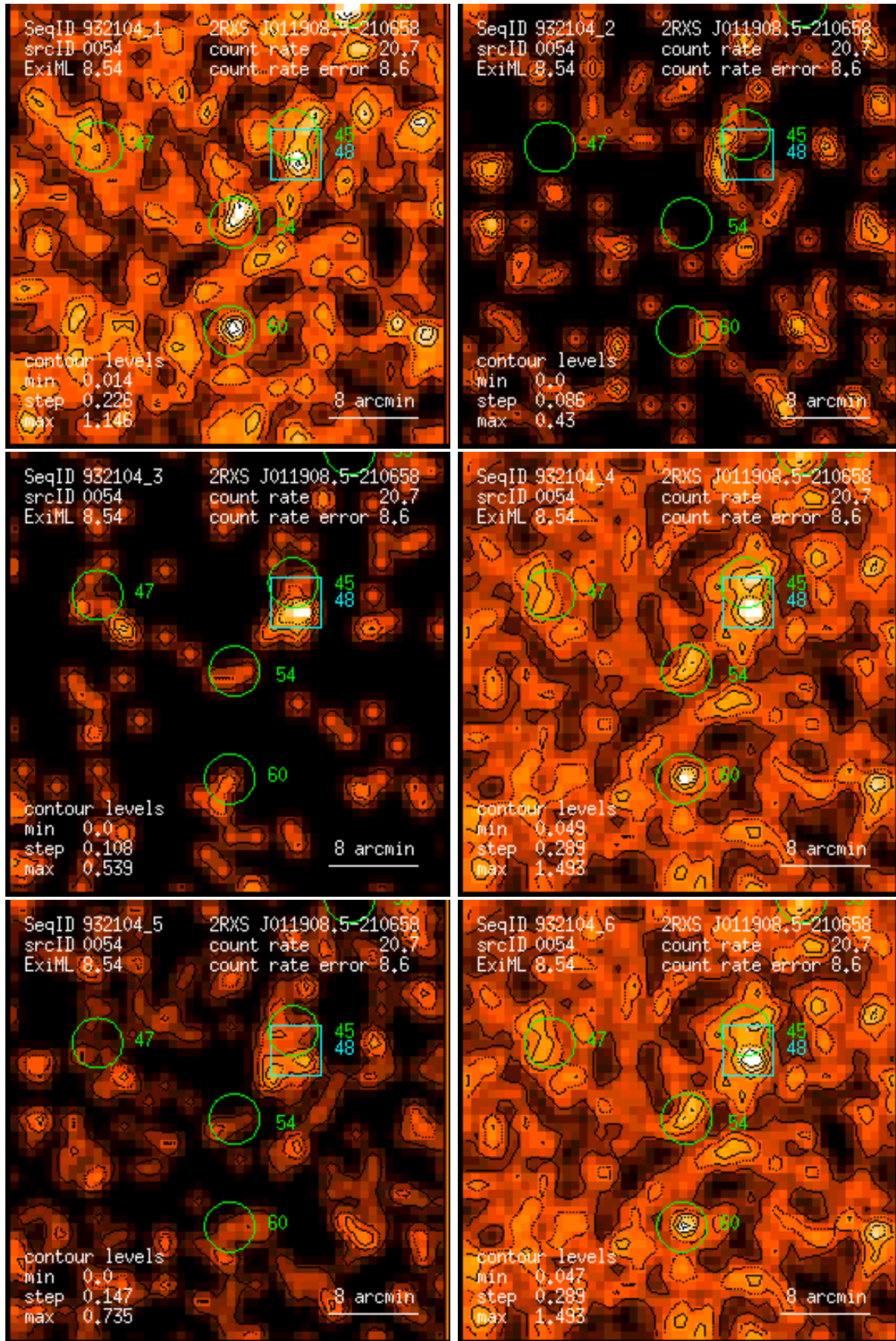
Figure 54: RASS 932104: detection 0054: band rate images, Gaussian filter: (1) PSPC channels 11 – 41, (2) 52 – 90, (3) 91 – 201, (4) 11 – 235, (5) 52 – 201, (6) 11 – 201. Broad band rates in counts/ks. Band rate contour levels in counts/ks/arcmin 2 .
