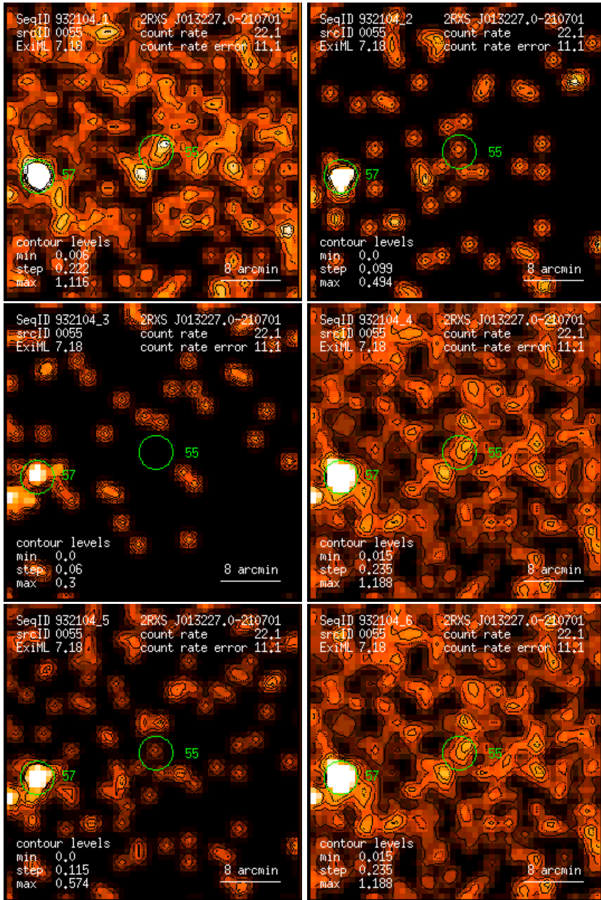
Figure 55: RASS 932104: detection 0055: band rate images, Gaussian filter: (1) PSPC channels 11 – 41, (2) 52 – 90, (3) 91 – 201, (4) 11 – 235, (5) 52 – 201, (6) 11 – 201. Broad band rates in counts/ks. Band rate contour levels in counts/ks/arcmin 2 .
