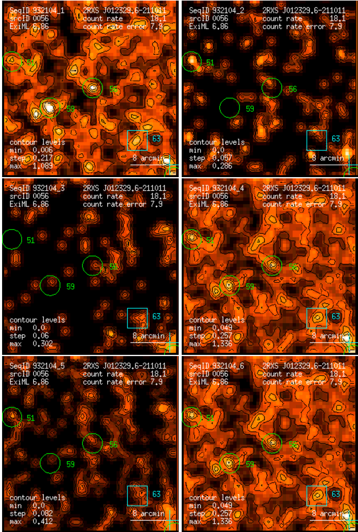
Figure 56: RASS 932104: detection 0056: band rate images, Gaussian filter: (1) PSPC channels 11 – 41, (2) 52 – 90, (3) 91 – 201, (4) 11 – 235, (5) 52 – 201, (6) 11 – 201. Broad band rates in counts/ks. Band rate contour levels in counts/ks/arcmin 2 .
