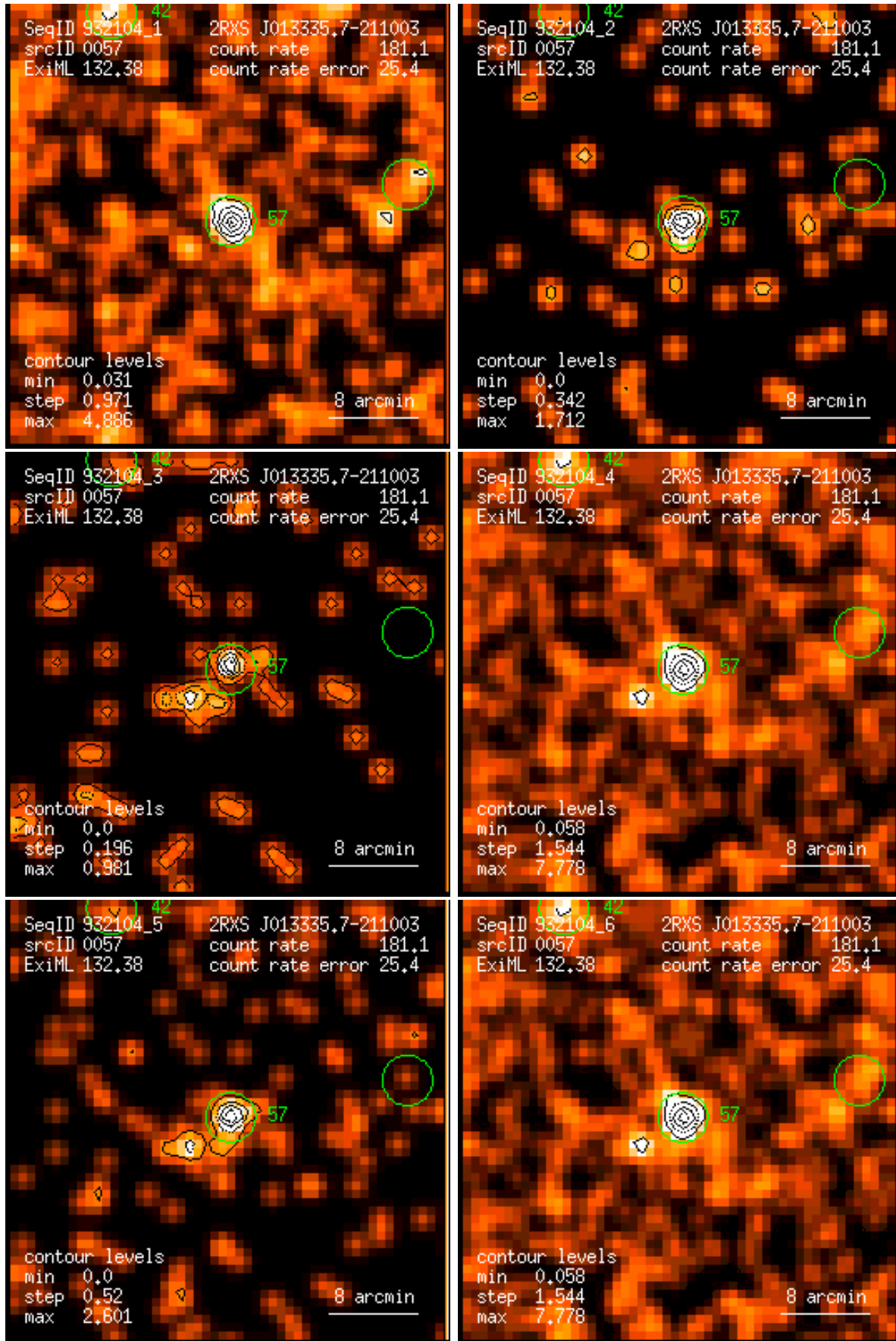
Figure 57: RASS 932104: detection 0057: band rate images, Gaussian filter: (1) PSPC channels 11 – 41, (2) 52 – 90, (3) 91 – 201, (4) 11 – 235, (5) 52 – 201, (6) 11 – 201. Broad band rates in counts/ks. Band rate contour levels in counts/ks/arcmin 2 .
